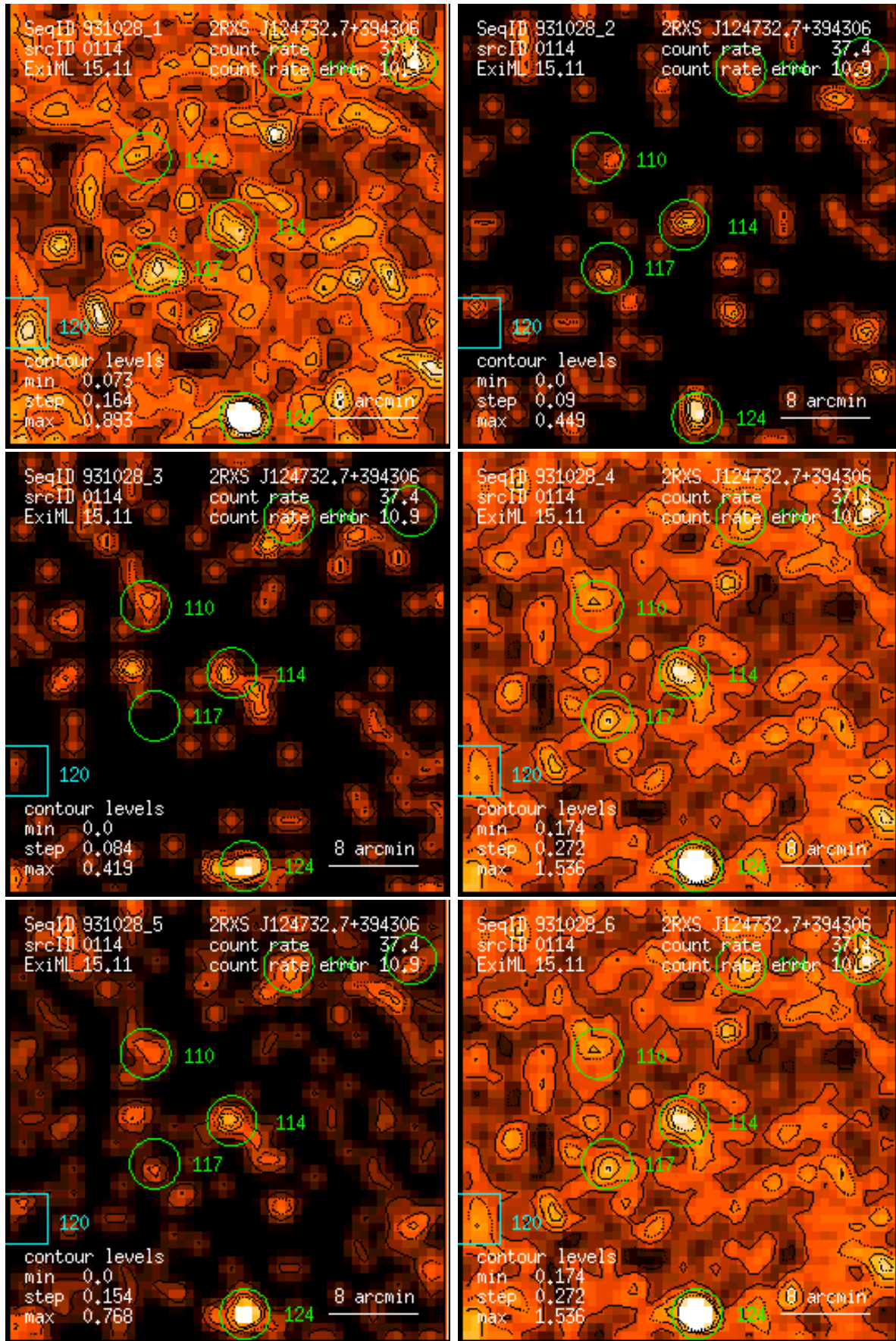
Figure 114: RASS 931028: detection 0114: band rate images, Gaussian filter: (1) PSPC channels 11 – 41, (2) 52 – 90, (3) 91 – 201, (4) 11 – 235, (5) 52 – 201, (6) 11 – 201. Broad band rates in counts/ks. Band rate contour levels in counts/ks/arcmin 2 .
