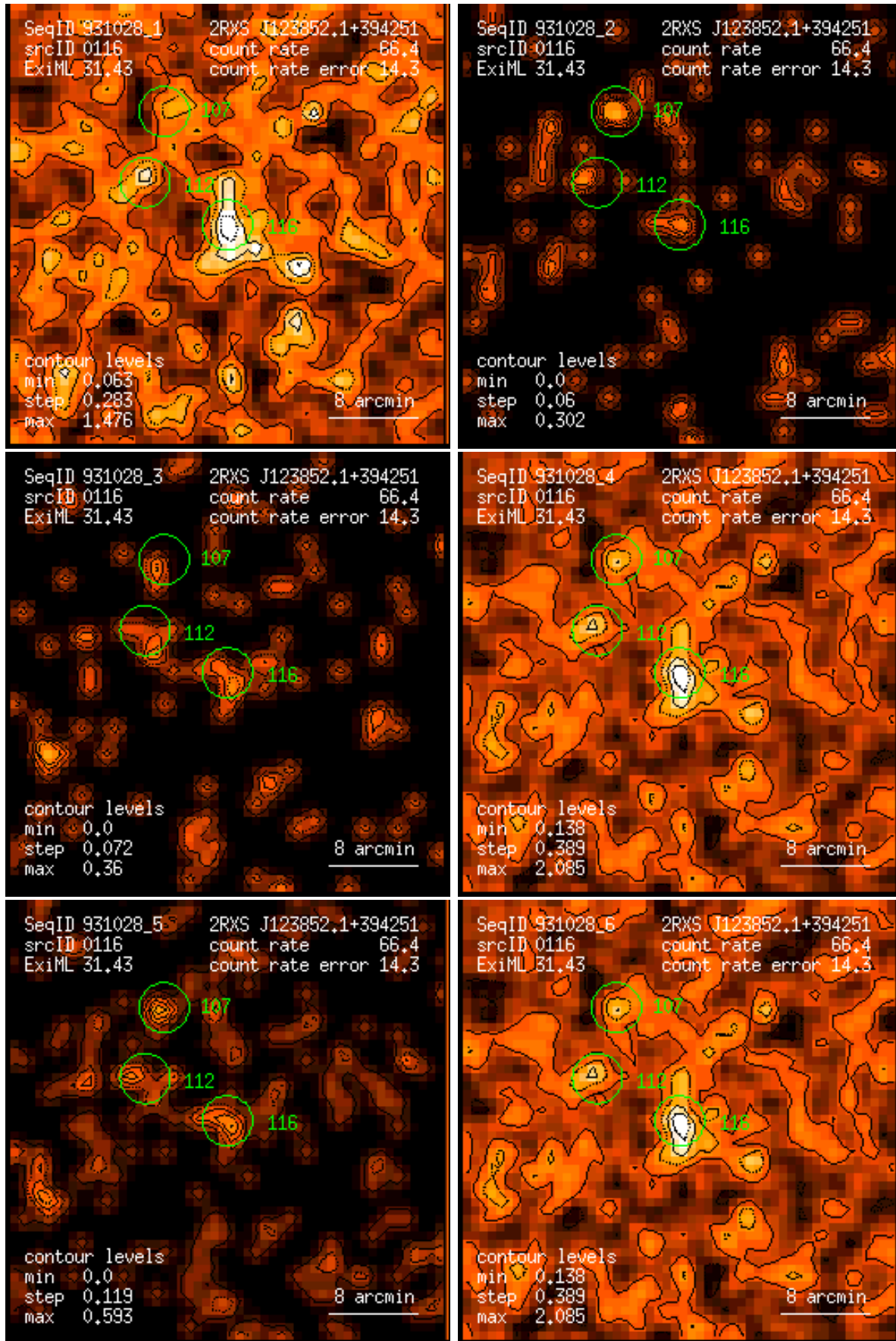
Figure 116: RASS 931028: detection 0116: band rate images, Gaussian filter: (1) PSPC channels 11 – 41, (2) 52 – 90, (3) 91 – 201, (4) 11 – 235, (5) 52 – 201, (6) 11 – 201. Broad band rates in counts/ks. Band rate contour levels in counts/ks/arcmin 2 .
