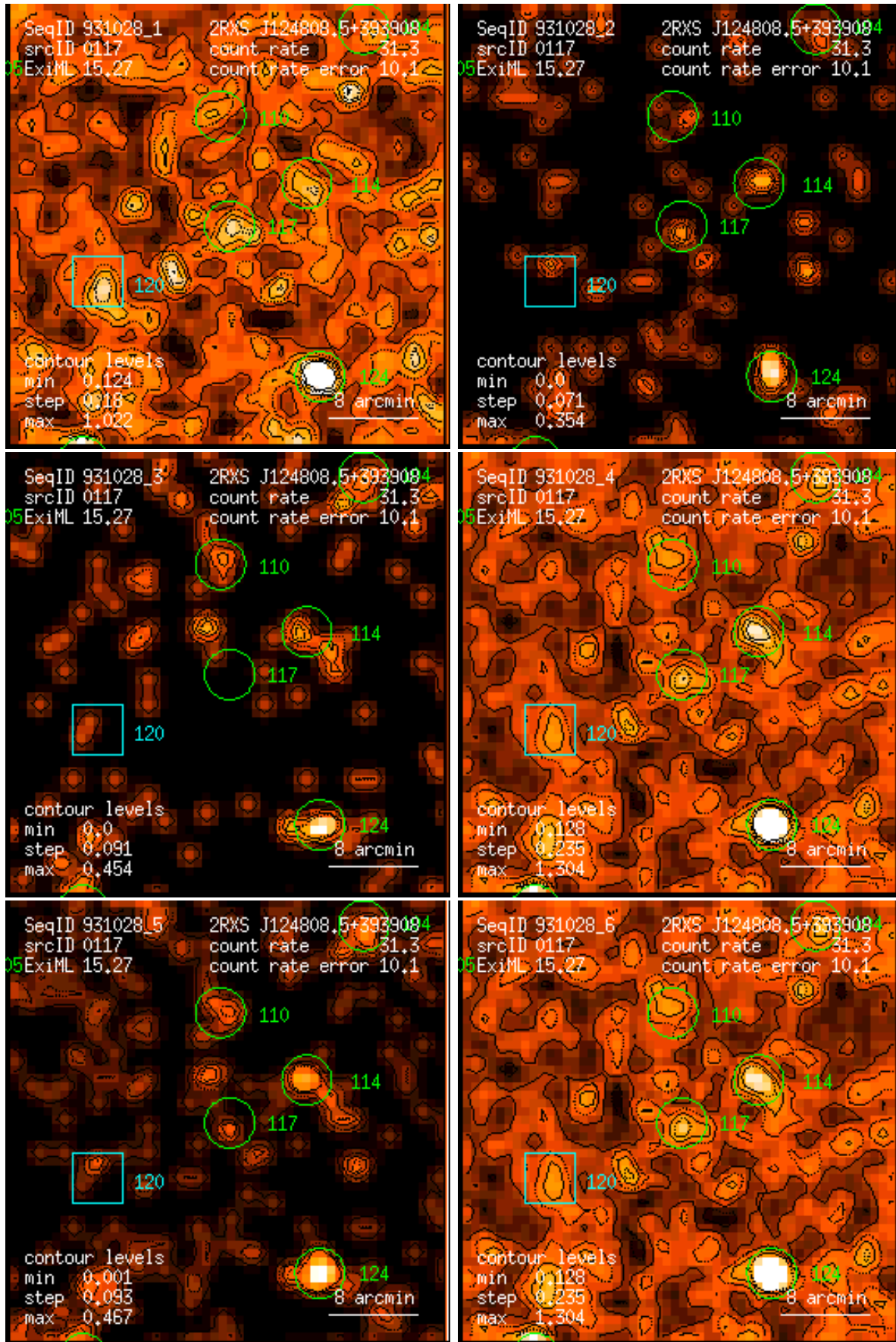
Figure 117: RASS 931028: detection 0117: band rate images, Gaussian filter: (1) PSPC channels 11 – 41, (2) 52 – 90, (3) 91 – 201, (4) 11 – 235, (5) 52 – 201, (6) 11 – 201. Broad band rates in counts/ks. Band rate contour levels in counts/ks/arcmin 2 .
