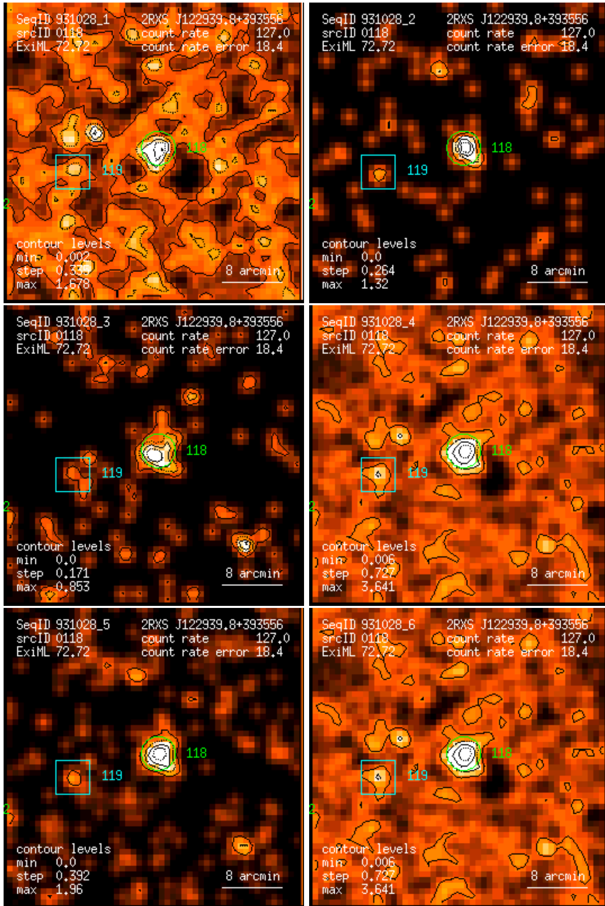
Figure 118: RASS 931028: detection 0118: band rate images, Gaussian filter: (1) PSPC channels 11 – 41, (2) 52 – 90, (3) 91 – 201, (4) 11 – 235, (5) 52 – 201, (6) 11 – 201. Broad band rates in counts/ks. Band rate contour levels in counts/ks/arcmin 2 .
