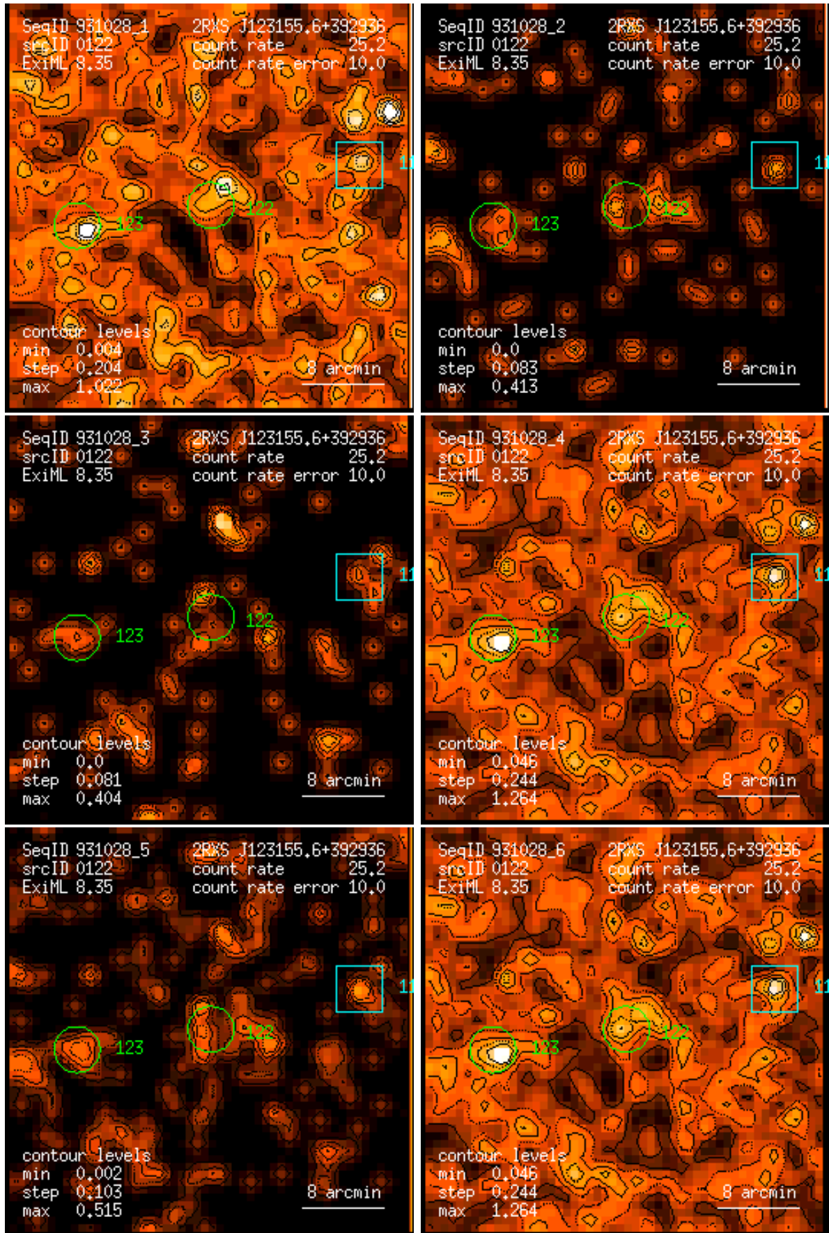
Figure 122: RASS 931028: detection 0122: band rate images, Gaussian filter: (1) PSPC channels 11 – 41, (2) 52 – 90, (3) 91 – 201, (4) 11 – 235, (5) 52 – 201, (6) 11 – 201. Broad band rates in counts/ks. Band rate contour levels in counts/ks/arcmin 2 .
