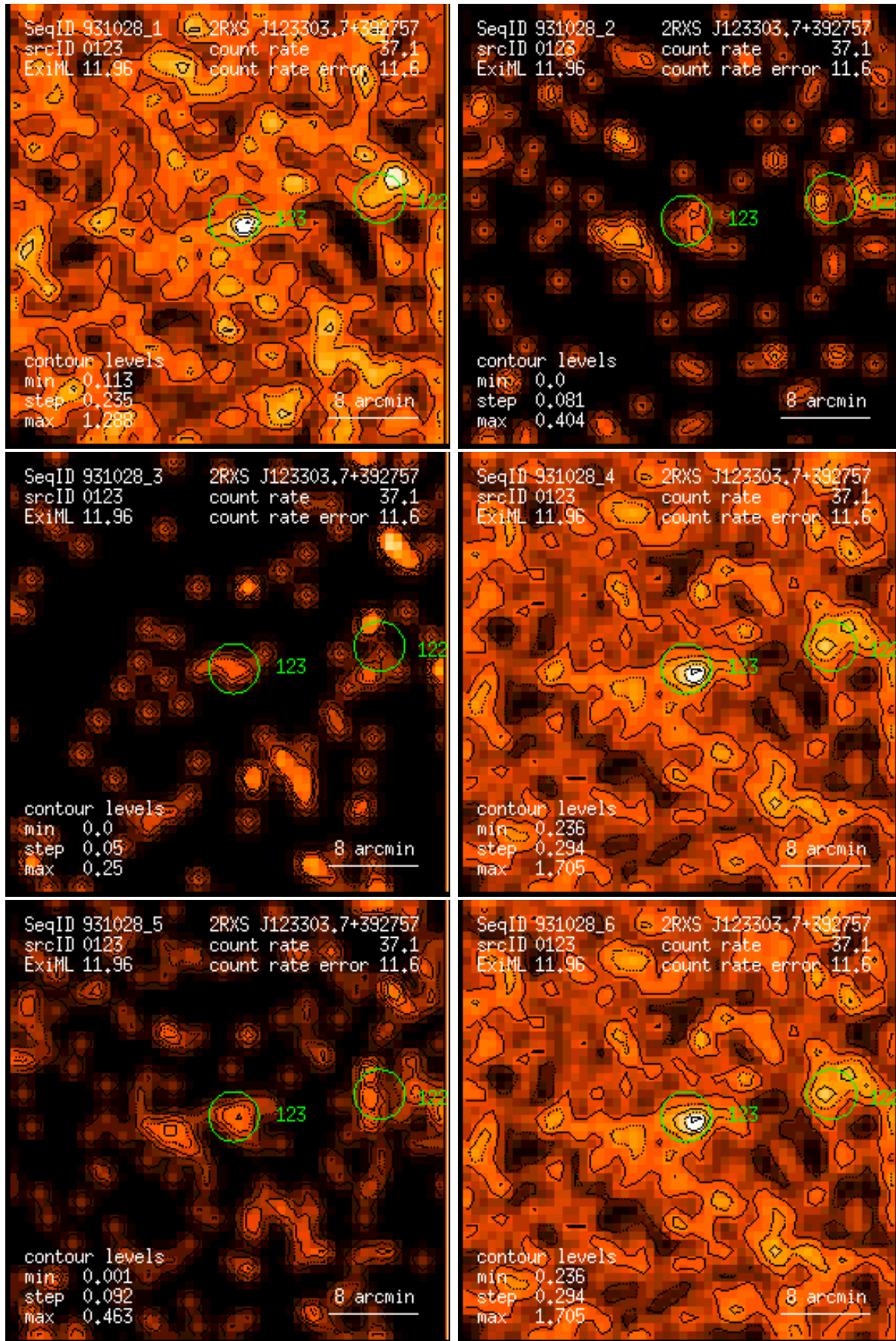
Figure 123: RASS 931028: detection 0123: band rate images, Gaussian filter: (1) PSPC channels 11 – 41, (2) 52 – 90, (3) 91 – 201, (4) 11 – 235, (5) 52 – 201, (6) 11 – 201. Broad band rates in counts/ks. Band rate contour levels in counts/ks/arcmin 2 .
