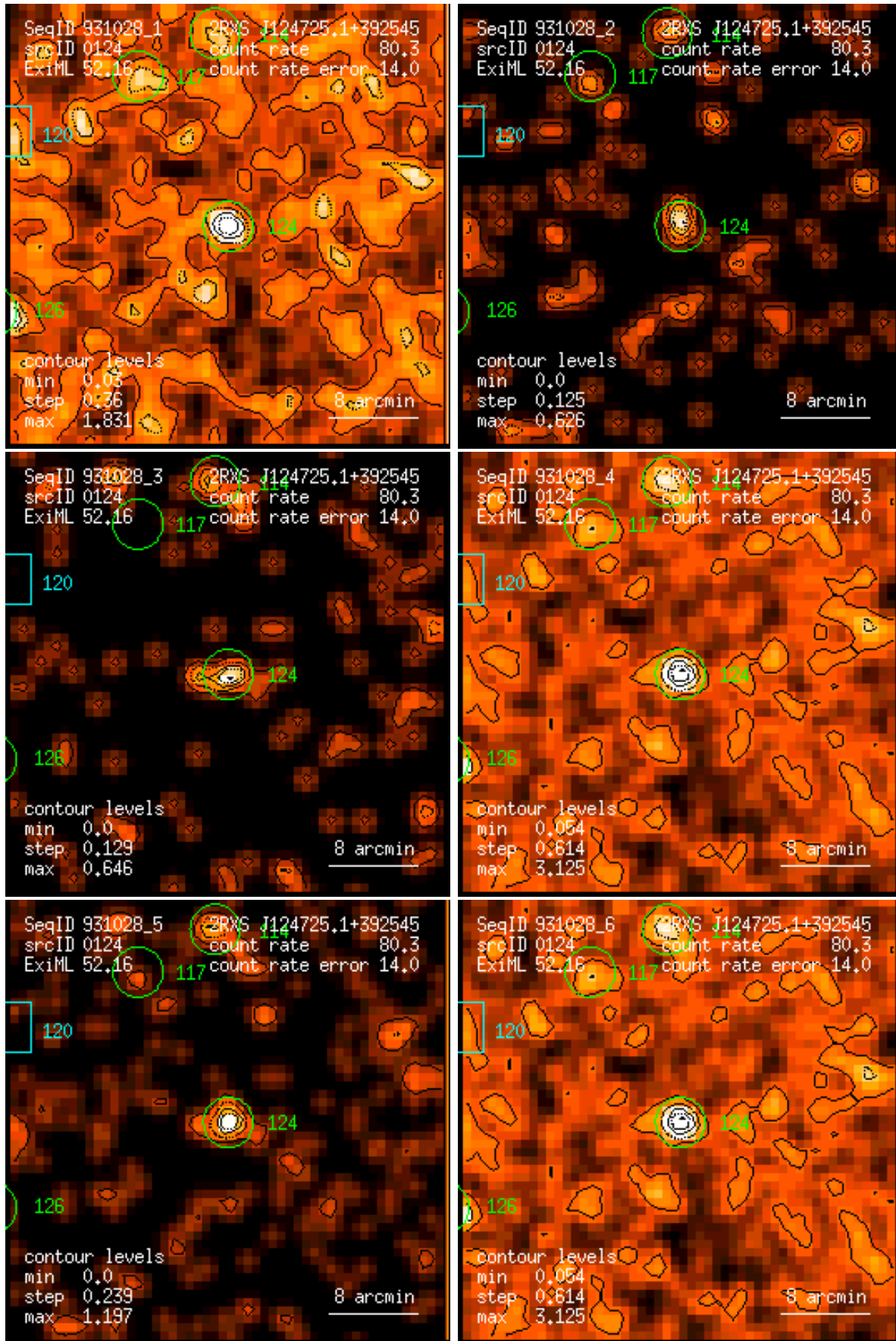
Figure 124: RASS 931028: detection 0124: band rate images, Gaussian filter: (1) PSPC channels 11 – 41, (2) 52 – 90, (3) 91 – 201, (4) 11 – 235, (5) 52 – 201, (6) 11 – 201. Broad band rates in counts/ks. Band rate contour levels in counts/ks/arcmin 2 .
