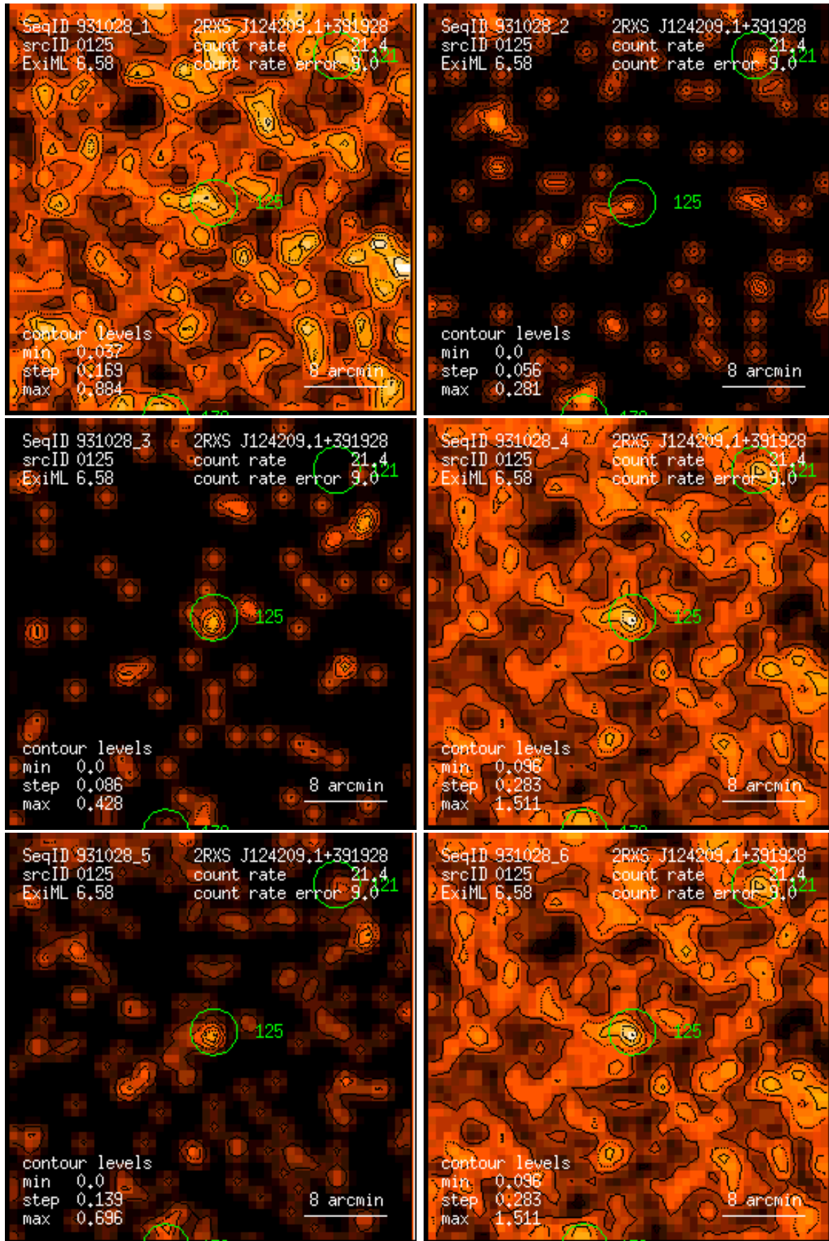
Figure 125: RASS 931028: detection 0125: band rate images, Gaussian filter: (1) PSPC channels 11 – 41, (2) 52 – 90, (3) 91 – 201, (4) 11 – 235, (5) 52 – 201, (6) 11 – 201. Broad band rates in counts/ks. Band rate contour levels in counts/ks/arcmin 2 .
