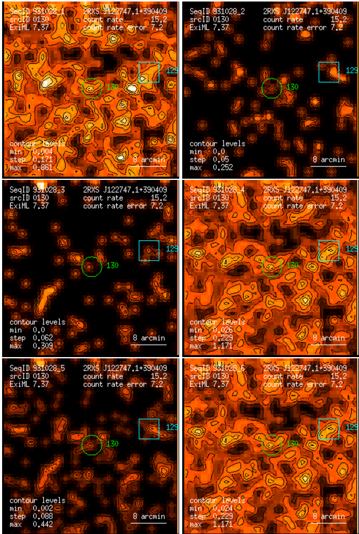
Figure 130: RASS 931028: detection 0130: band rate images, Gaussian filter: (1) PSPC channels 11 – 41, (2) 52 – 90, (3) 91 – 201, (4) 11 – 235, (5) 52 – 201, (6) 11 – 201. Broad band rates in counts/ks. Band rate contour levels in counts/ks/arcmin 2 .
