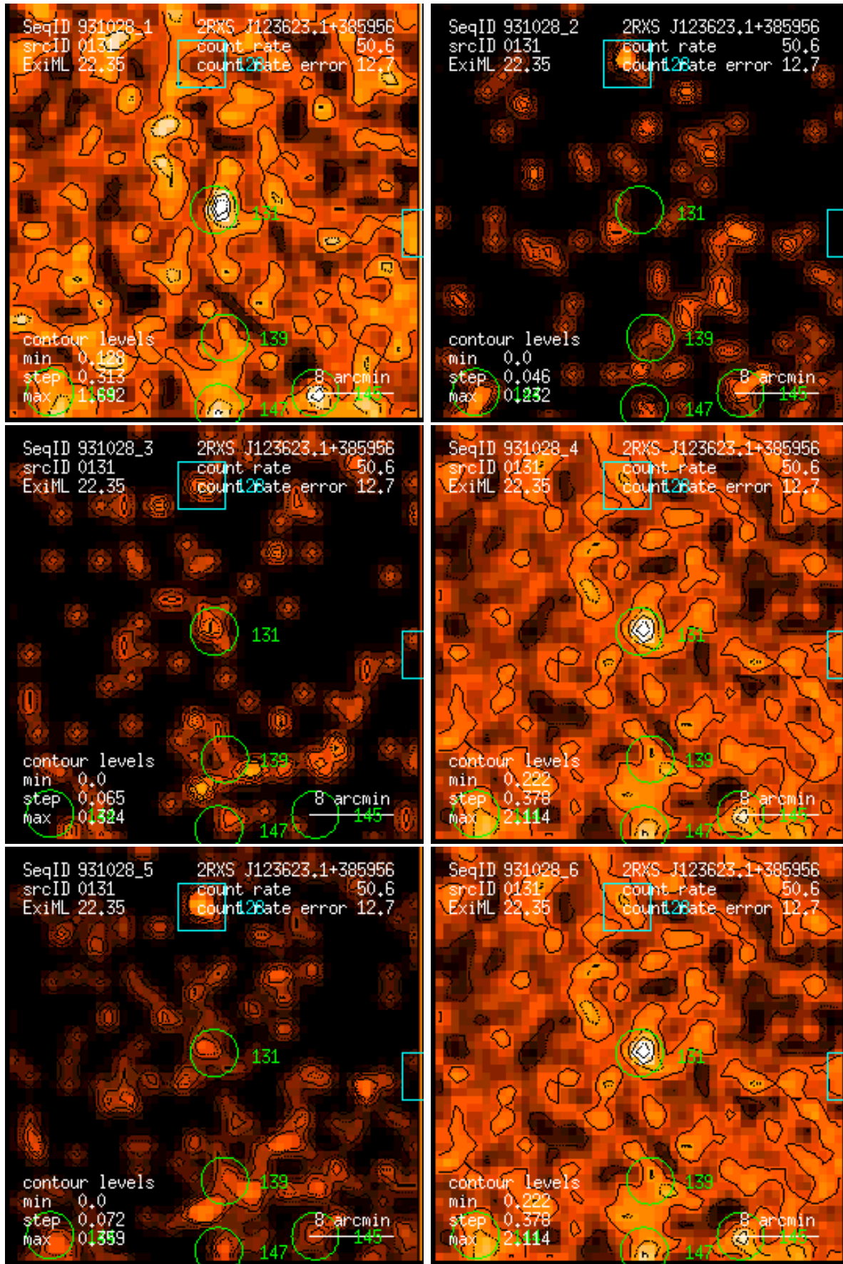
Figure 131: RASS 931028: detection 0131: band rate images, Gaussian filter: (1) PSPC channels 11 – 41, (2) 52 – 90, (3) 91 – 201, (4) 11 – 235, (5) 52 – 201, (6) 11 – 201. Broad band rates in counts/ks. Band rate contour levels in counts/ks/arcmin 2 .
