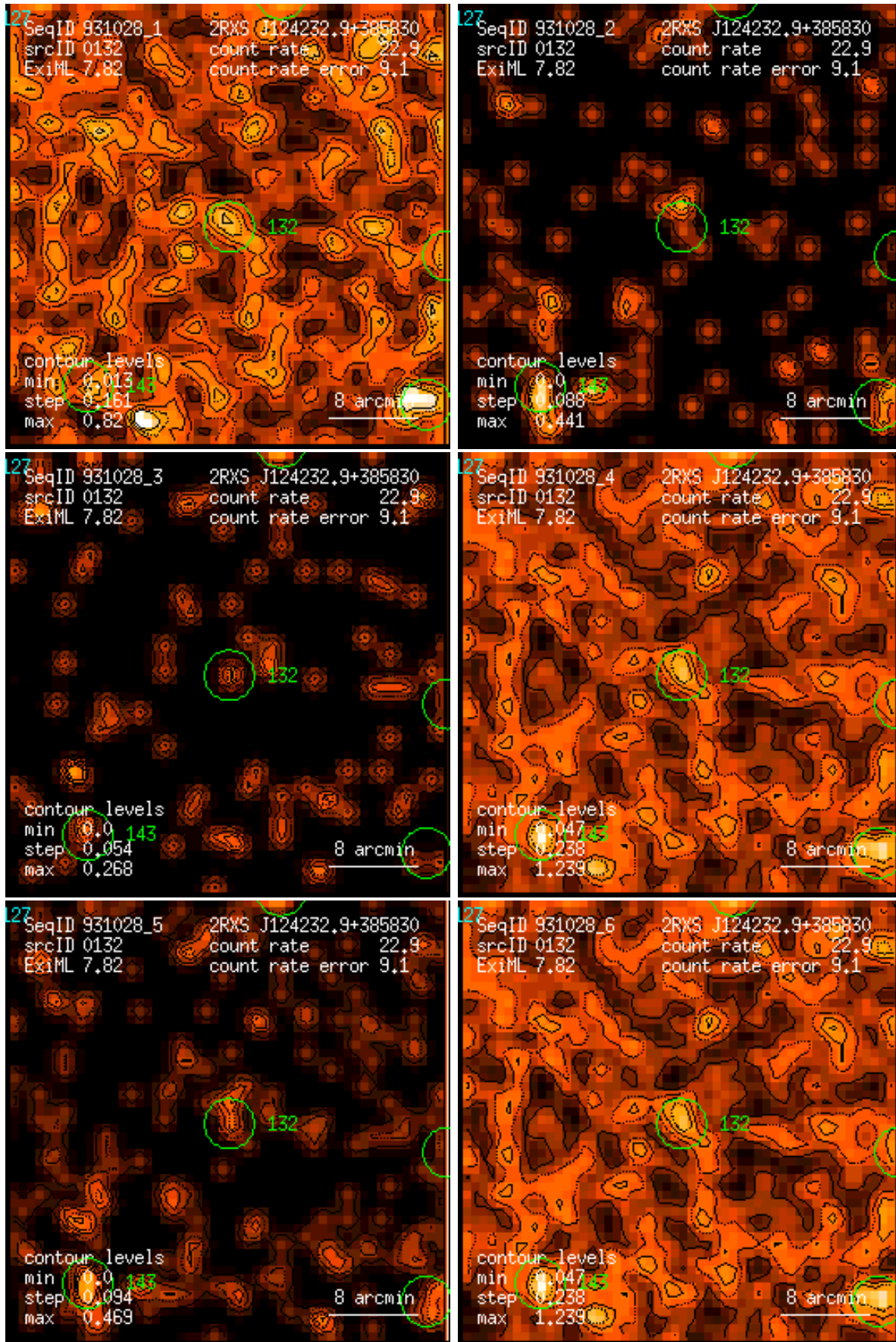
Figure 132: RASS 931028: detection 0132: band rate images, Gaussian filter: (1) PSPC channels 11 – 41, (2) 52 – 90, (3) 91 – 201, (4) 11 – 235, (5) 52 – 201, (6) 11 – 201. Broad band rates in counts/ks. Band rate contour levels in counts/ks/arcmin 2 .
