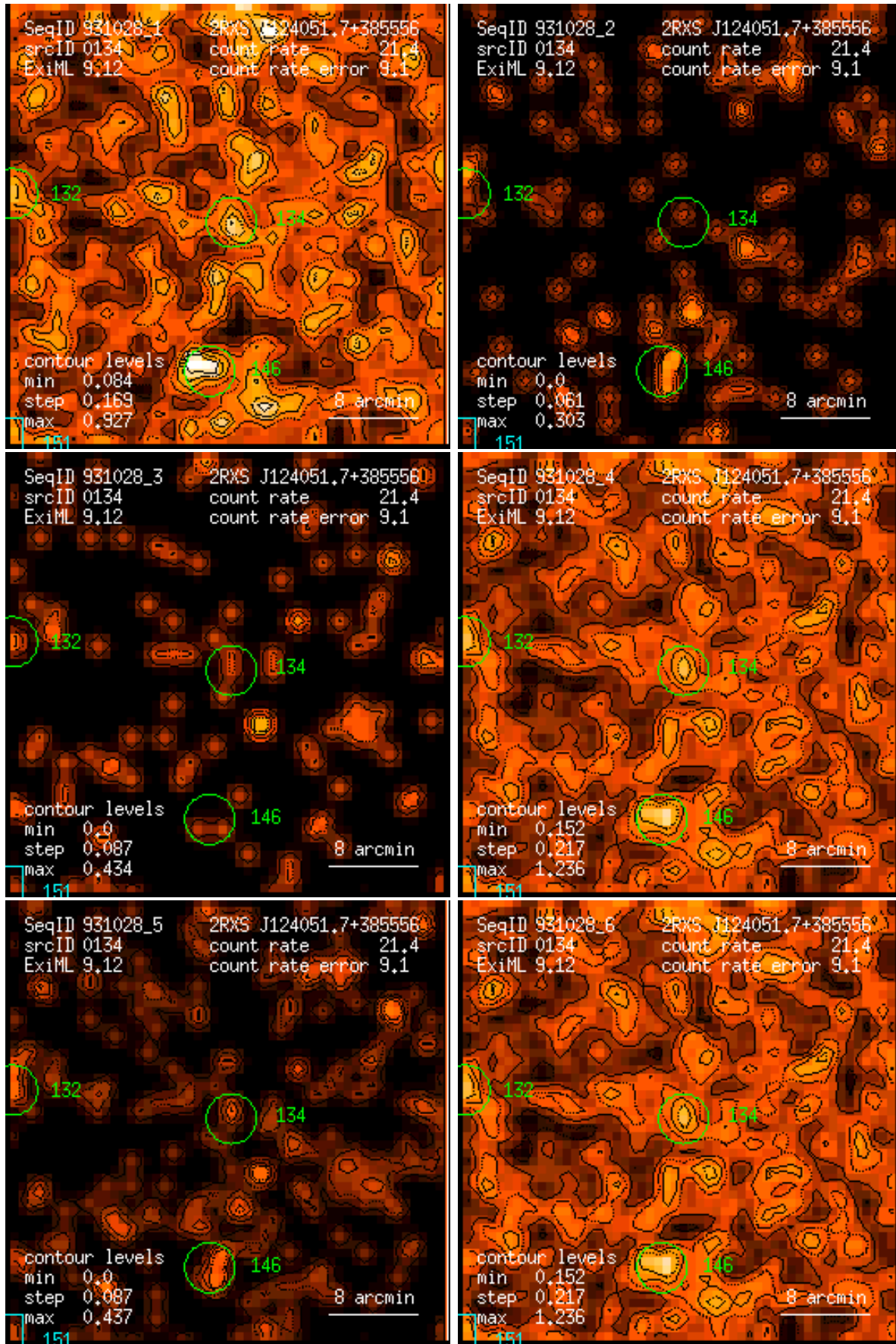
Figure 134: RASS 931028: detection 0134: band rate images, Gaussian filter: (1) PSPC channels 11 – 41, (2) 52 – 90, (3) 91 – 201, (4) 11 – 235, (5) 52 – 201, (6) 11 – 201. Broad band rates in counts/ks. Band rate contour levels in counts/ks/arcmin 2 .
