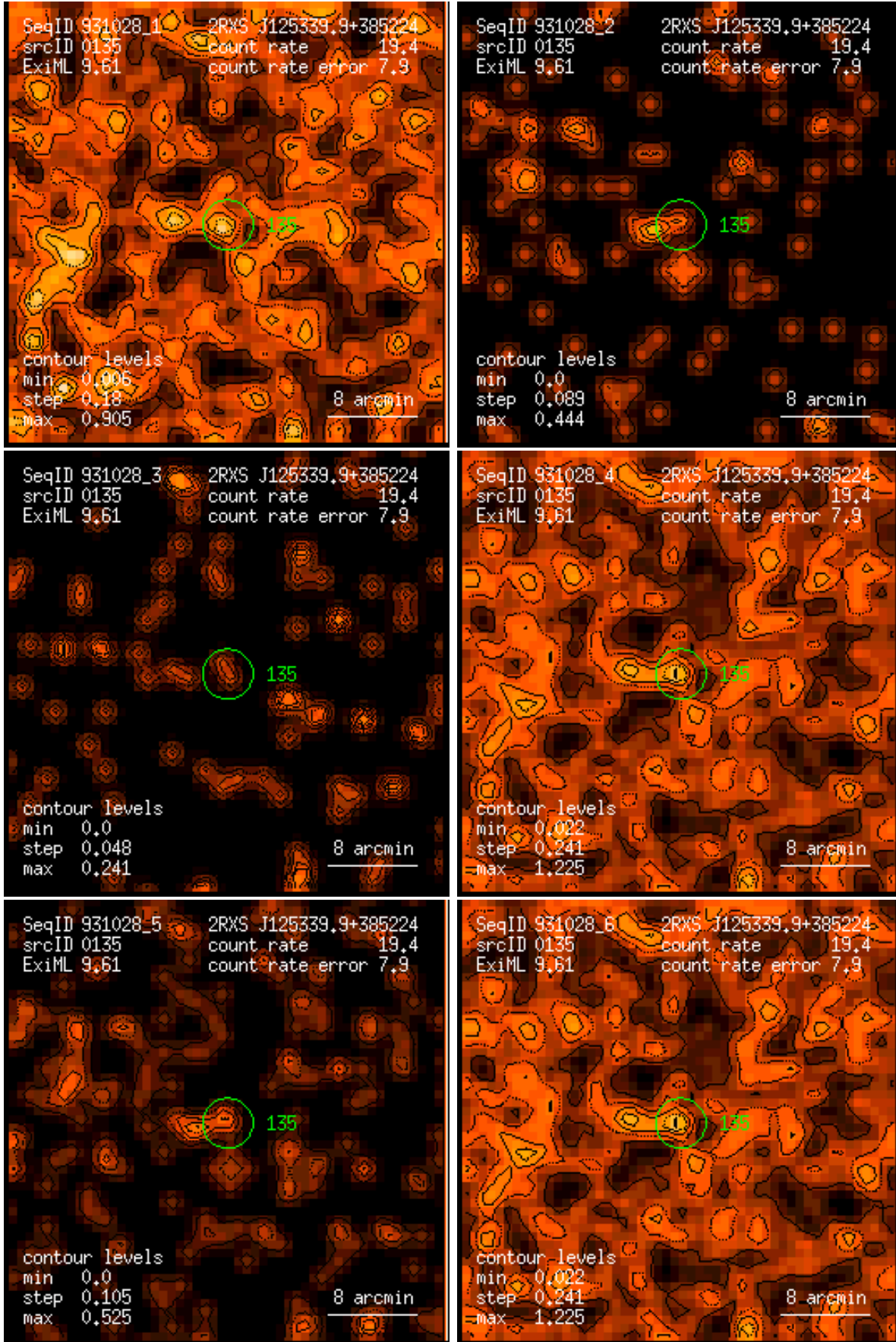
Figure 135: RASS 931028: detection 0135: band rate images, Gaussian filter: (1) PSPC channels 11 – 41, (2) 52 – 90, (3) 91 – 201, (4) 11 – 235, (5) 52 – 201, (6) 11 – 201. Broad band rates in counts/ks. Band rate contour levels in counts/ks/arcmin 2 .
