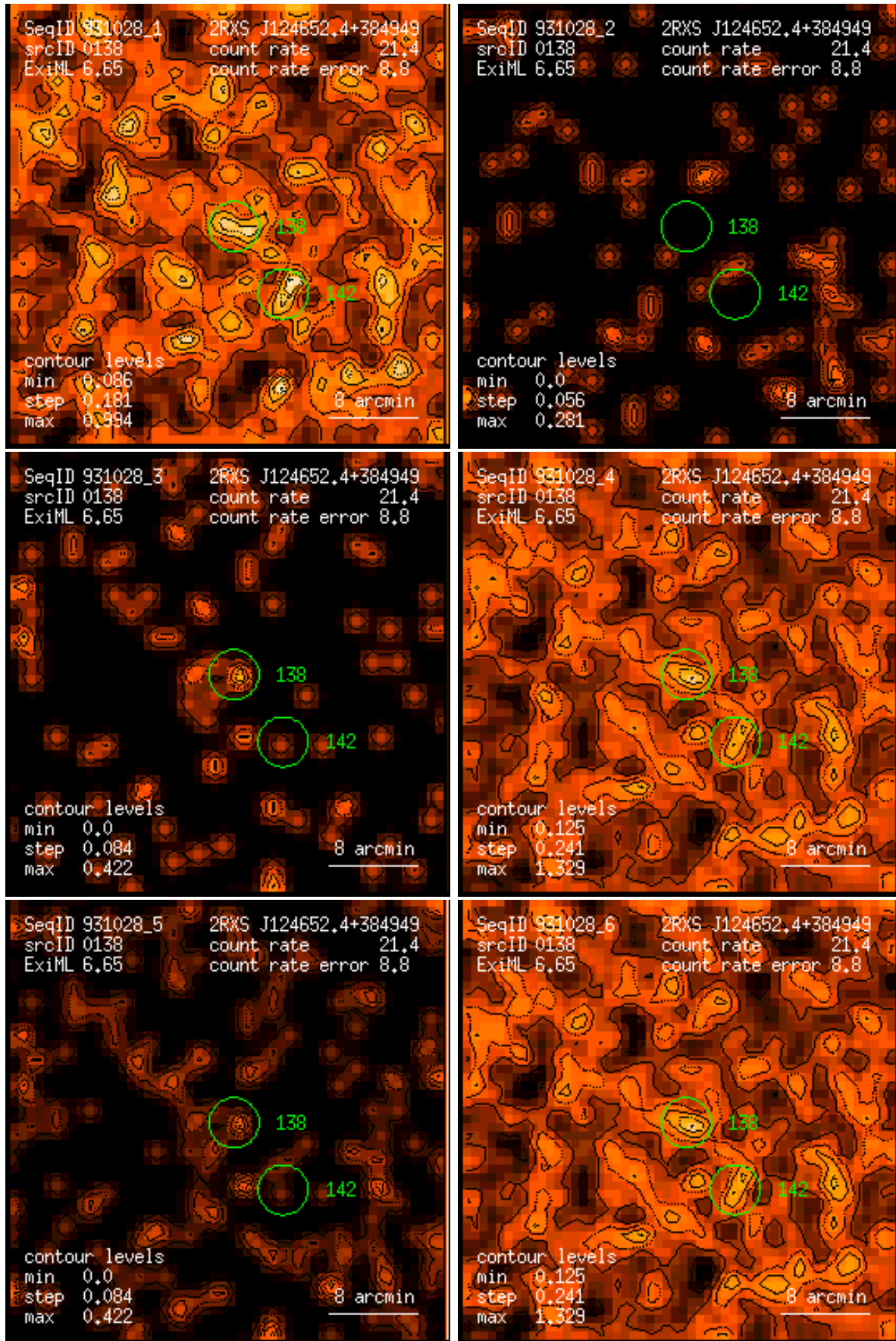
Figure 138: RASS 931028: detection 0138: band rate images, Gaussian filter: (1) PSPC channels 11 – 41, (2) 52 – 90, (3) 91 – 201, (4) 11 – 235, (5) 52 – 201, (6) 11 – 201. Broad band rates in counts/ks. Band rate contour levels in counts/ks/arcmin 2 .
