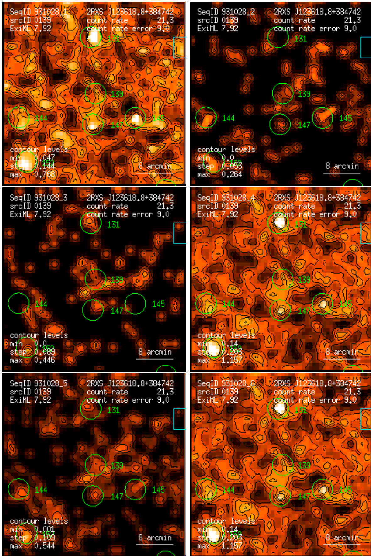
Figure 139: RASS 931028: detection 0139: band rate images, Gaussian filter: (1) PSPC channels 11 – 41, (2) 52 – 90, (3) 91 – 201, (4) 11 – 235, (5) 52 – 201, (6) 11 – 201. Broad band rates in counts/ks. Band rate contour levels in counts/ks/arcmin 2 .
