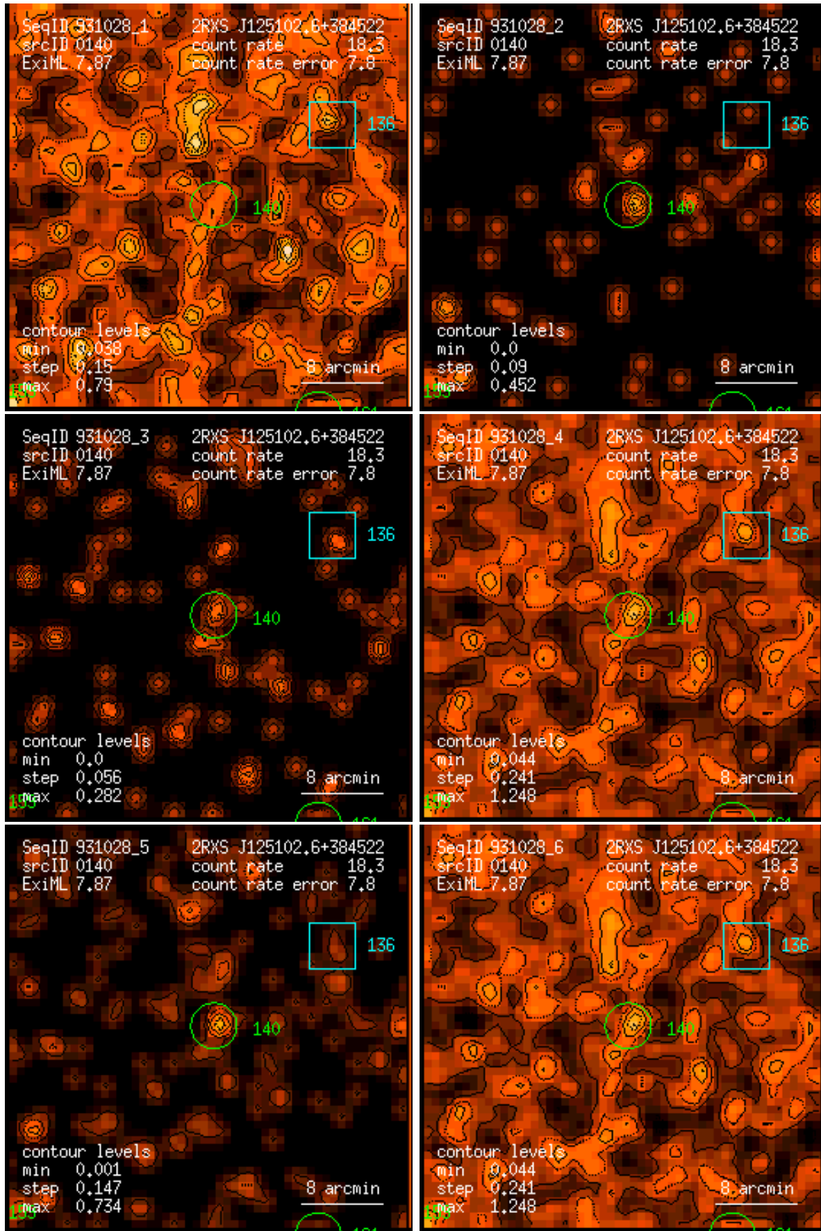
Figure 140: RASS 931028: detection 0140: band rate images, Gaussian filter: (1) PSPC channels 11 – 41, (2) 52 – 90, (3) 91 – 201, (4) 11 – 235, (5) 52 – 201, (6) 11 – 201. Broad band rates in counts/ks. Band rate contour levels in counts/ks/arcmin 2 .
