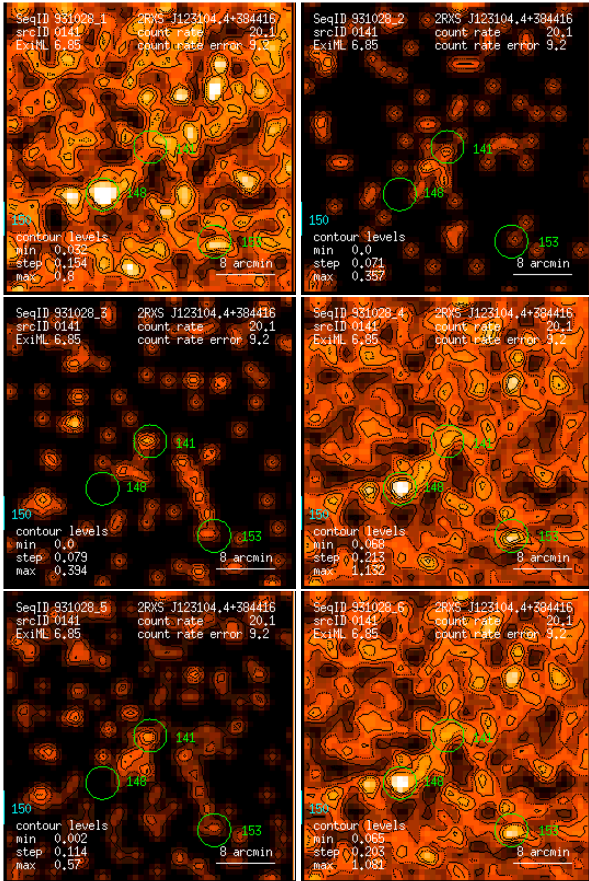
Figure 141: RASS 931028: detection 0141: band rate images, Gaussian filter: (1) PSPC channels 11 – 41, (2) 52 – 90, (3) 91 – 201, (4) 11 – 235, (5) 52 – 201, (6) 11 – 201. Broad band rates in counts/ks. Band rate contour levels in counts/ks/arcmin 2 .
