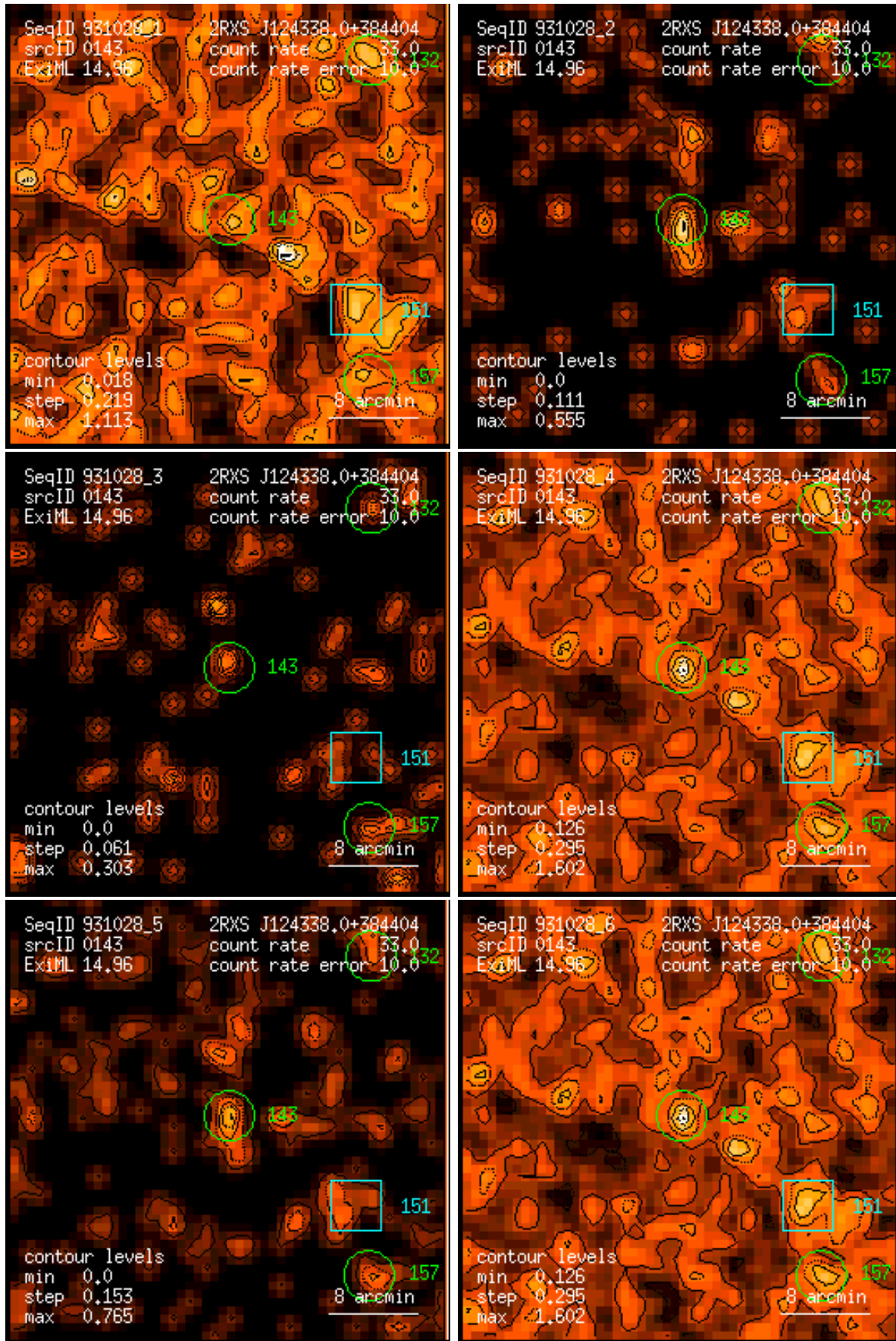
Figure 143: RASS 931028: detection 0143: band rate images, Gaussian filter: (1) PSPC channels 11 – 41, (2) 52 – 90, (3) 91 – 201, (4) 11 – 235, (5) 52 – 201, (6) 11 – 201. Broad band rates in counts/ks. Band rate contour levels in counts/ks/arcmin 2 .
