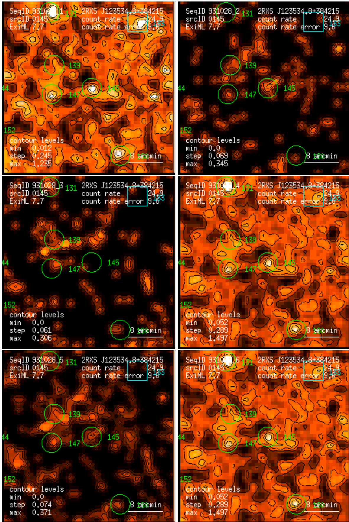
Figure 145: RASS 931028: detection 0145: band rate images, Gaussian filter: (1) PSPC channels 11 – 41, (2) 52 – 90, (3) 91 – 201, (4) 11 – 235, (5) 52 – 201, (6) 11 – 201. Broad band rates in counts/ks. Band rate contour levels in counts/ks/arcmin 2 .
