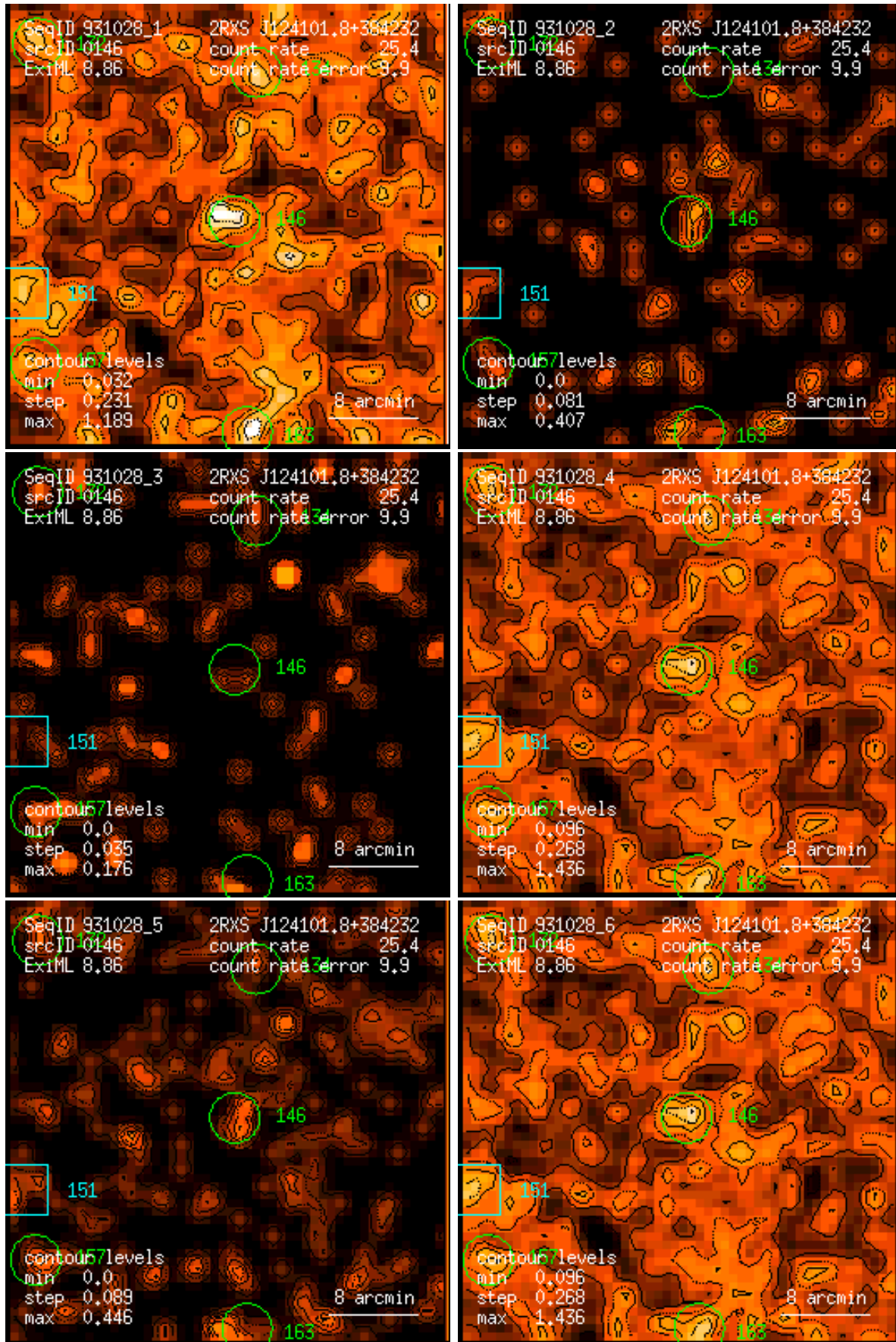
Figure 146: RASS 931028: detection 0146: band rate images, Gaussian filter: (1) PSPC channels 11 – 41, (2) 52 – 90, (3) 91 – 201, (4) 11 – 235, (5) 52 – 201, (6) 11 – 201. Broad band rates in counts/ks. Band rate contour levels in counts/ks/arcmin 2 .
