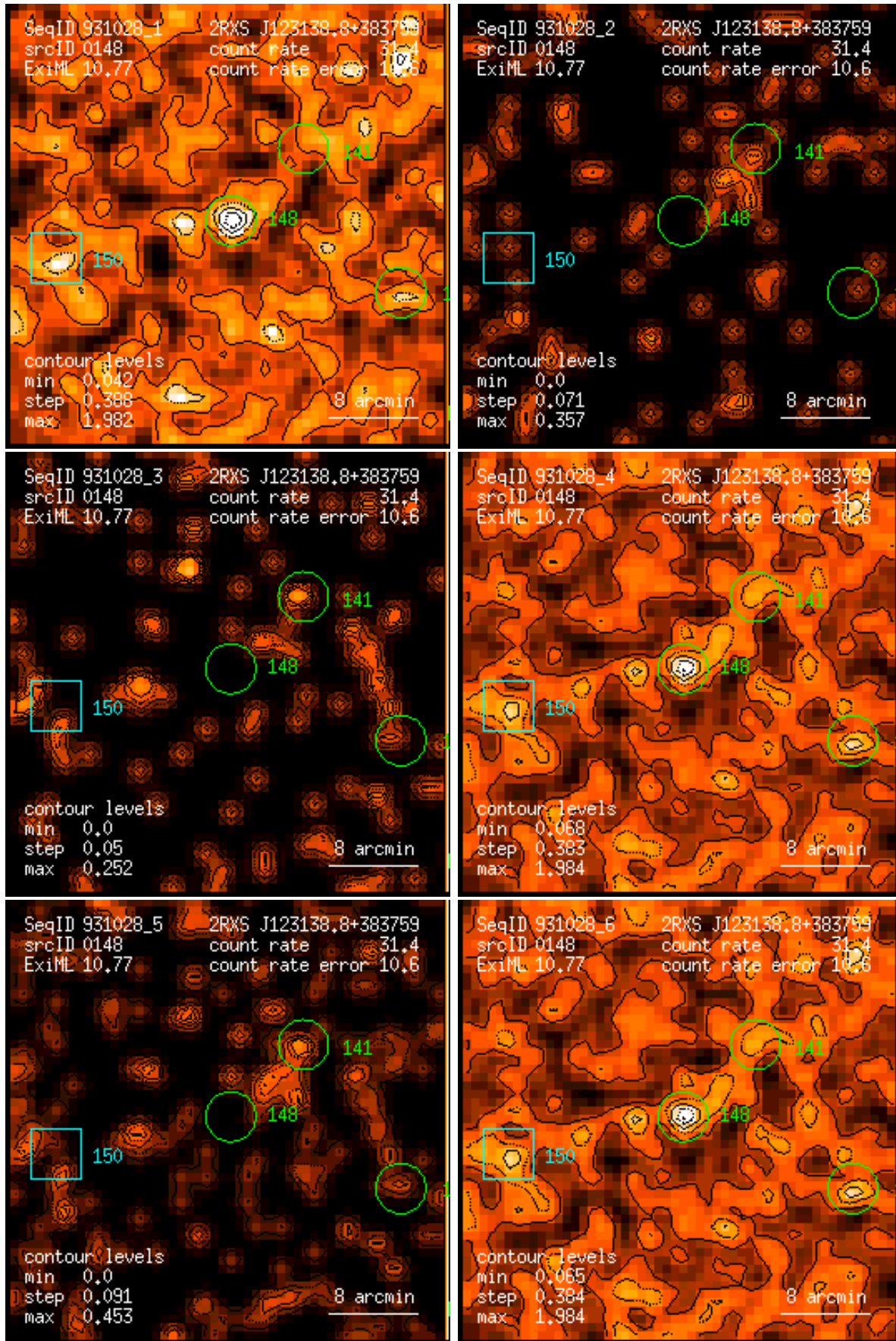
Figure 148: RASS 931028: detection 0148: band rate images, Gaussian filter: (1) PSPC channels 11 – 41, (2) 52 – 90, (3) 91 – 201, (4) 11 – 235, (5) 52 – 201, (6) 11 – 201. Broad band rates in counts/ks. Band rate contour levels in counts/ks/arcmin 2 .
