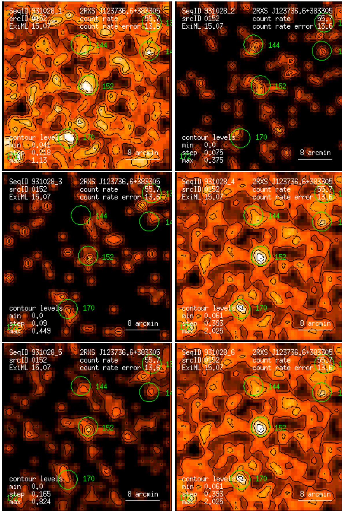
Figure 152: RASS 931028: detection 0152: band rate images, Gaussian filter: (1) PSPC channels 11 – 41, (2) 52 – 90, (3) 91 – 201, (4) 11 – 235, (5) 52 – 201, (6) 11 – 201. Broad band rates in counts/ks. Band rate contour levels in counts/ks/arcmin 2 .
