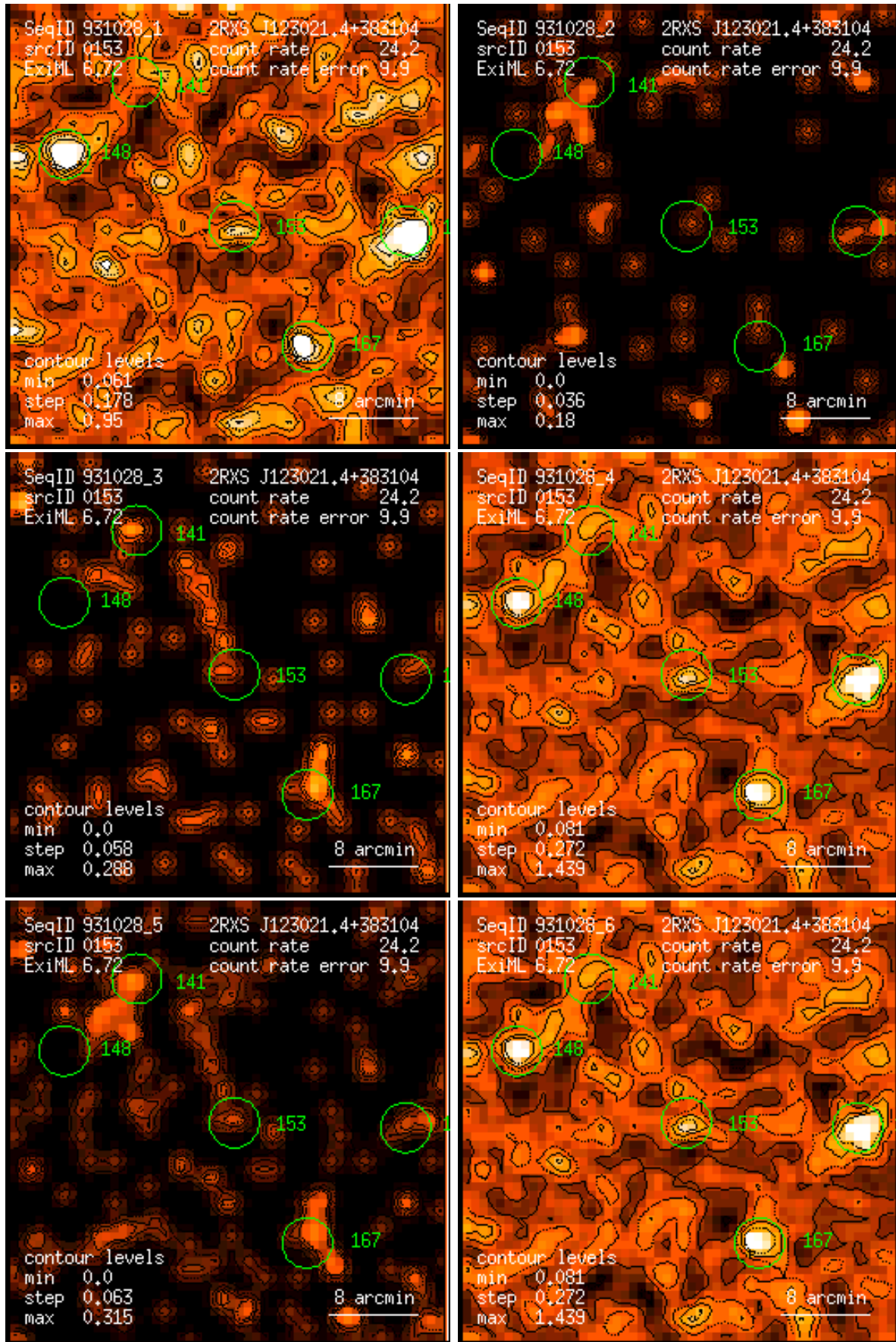
Figure 153: RASS 931028: detection 0153: band rate images, Gaussian filter: (1) PSPC channels 11 – 41, (2) 52 – 90, (3) 91 – 201, (4) 11 – 235, (5) 52 – 201, (6) 11 – 201. Broad band rates in counts/ks. Band rate contour levels in counts/ks/arcmin 2 .
