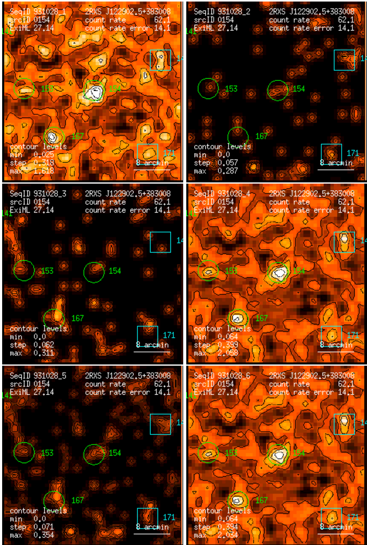
Figure 154: RASS 931028: detection 0154: band rate images, Gaussian filter: (1) PSPC channels 11 – 41, (2) 52 – 90, (3) 91 – 201, (4) 11 – 235, (5) 52 – 201, (6) 11 – 201. Broad band rates in counts/ks. Band rate contour levels in counts/ks/arcmin 2 .
