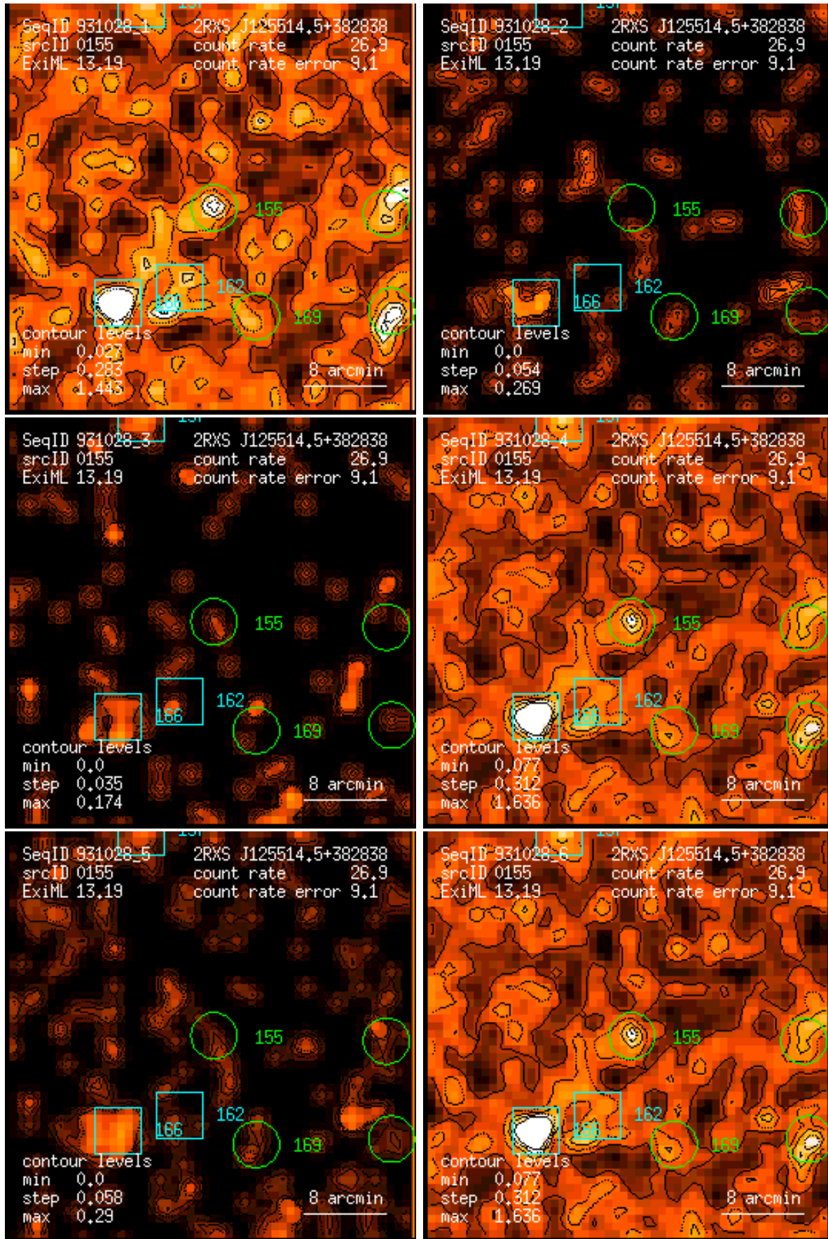
Figure 155: RASS 931028: detection 0155: band rate images, Gaussian filter: (1) PSPC channels 11 – 41, (2) 52 – 90, (3) 91 – 201, (4) 11 – 235, (5) 52 – 201, (6) 11 – 201. Broad band rates in counts/ks. Band rate contour levels in counts/ks/arcmin 2 .
