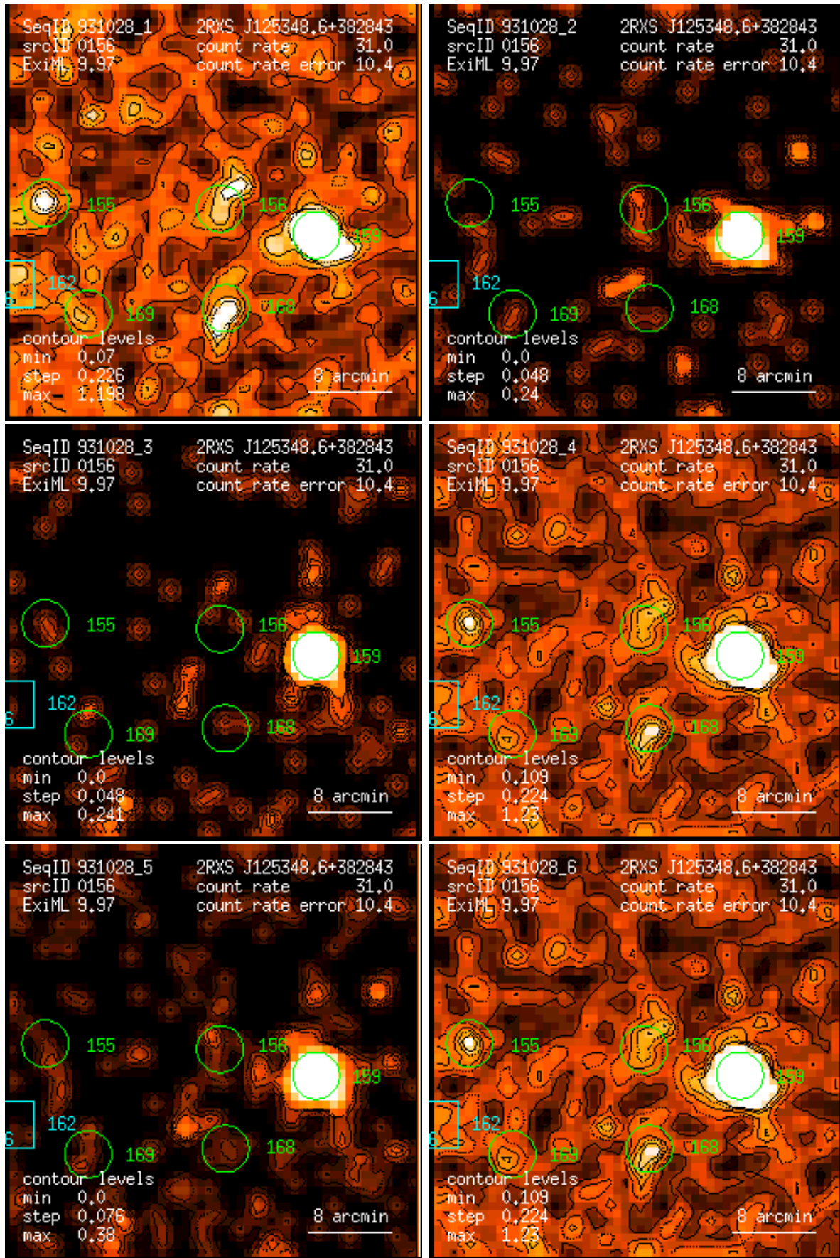
Figure 156: RASS 931028: detection 0156: band rate images, Gaussian filter: (1) PSPC channels 11 – 41, (2) 52 – 90, (3) 91 – 201, (4) 11 – 235, (5) 52 – 201, (6) 11 – 201. Broad band rates in counts/ks. Band rate contour levels in counts/ks/arcmin 2 .
