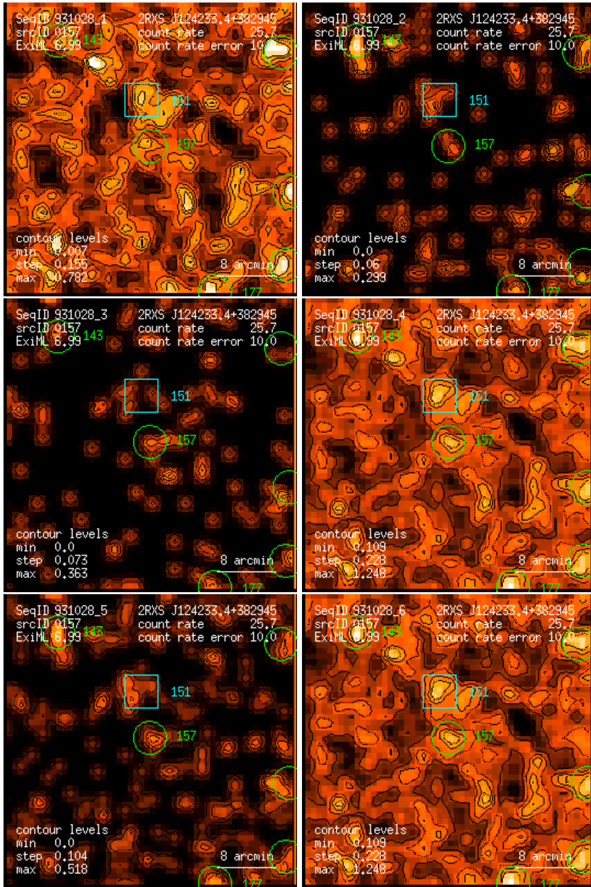
Figure 157: RASS 931028: detection 0157: band rate images, Gaussian filter: (1) PSPC channels 11 – 41, (2) 52 – 90, (3) 91 – 201, (4) 11 – 235, (5) 52 – 201, (6) 11 – 201. Broad band rates in counts/ks. Band rate contour levels in counts/ks/arcmin 2 .
