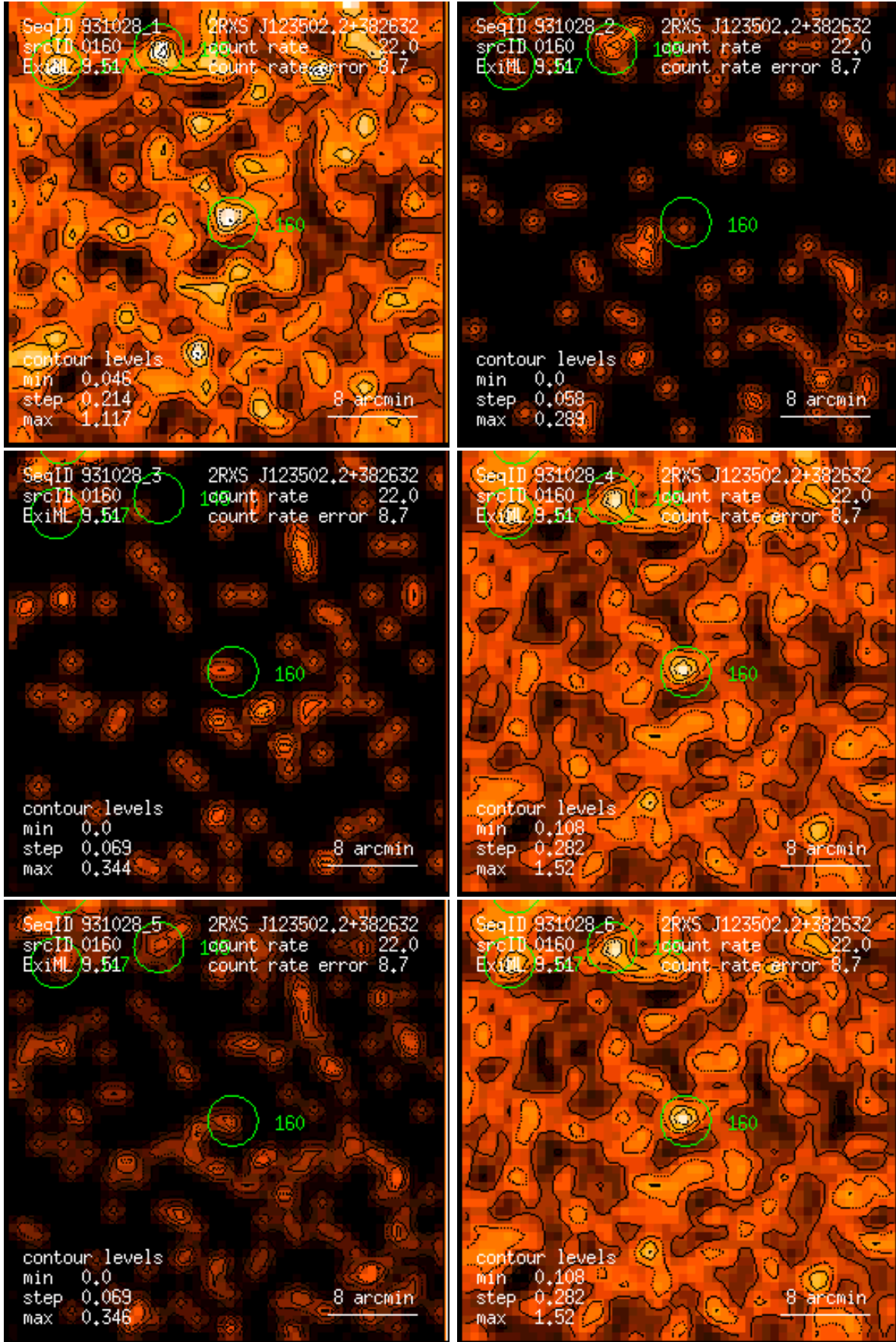
Figure 160: RASS 931028: detection 0160: band rate images, Gaussian filter: (1) PSPC channels 11 – 41, (2) 52 – 90, (3) 91 – 201, (4) 11 – 235, (5) 52 – 201, (6) 11 – 201. Broad band rates in counts/ks. Band rate contour levels in counts/ks/arcmin 2 .
