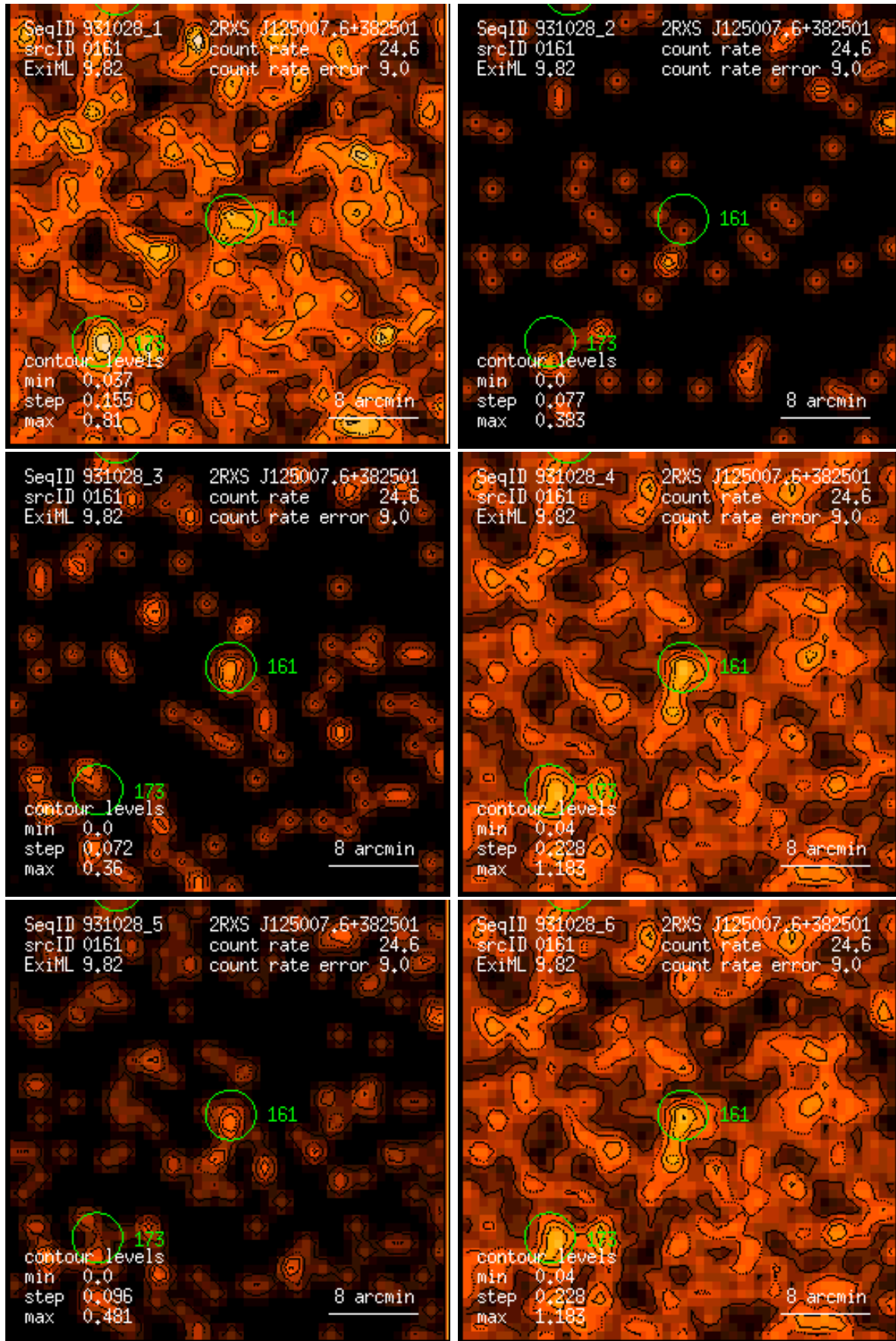
Figure 161: RASS 931028: detection 0161: band rate images, Gaussian filter: (1) PSPC channels 11 – 41, (2) 52 – 90, (3) 91 – 201, (4) 11 – 235, (5) 52 – 201, (6) 11 – 201. Broad band rates in counts/ks. Band rate contour levels in counts/ks/arcmin 2 .
