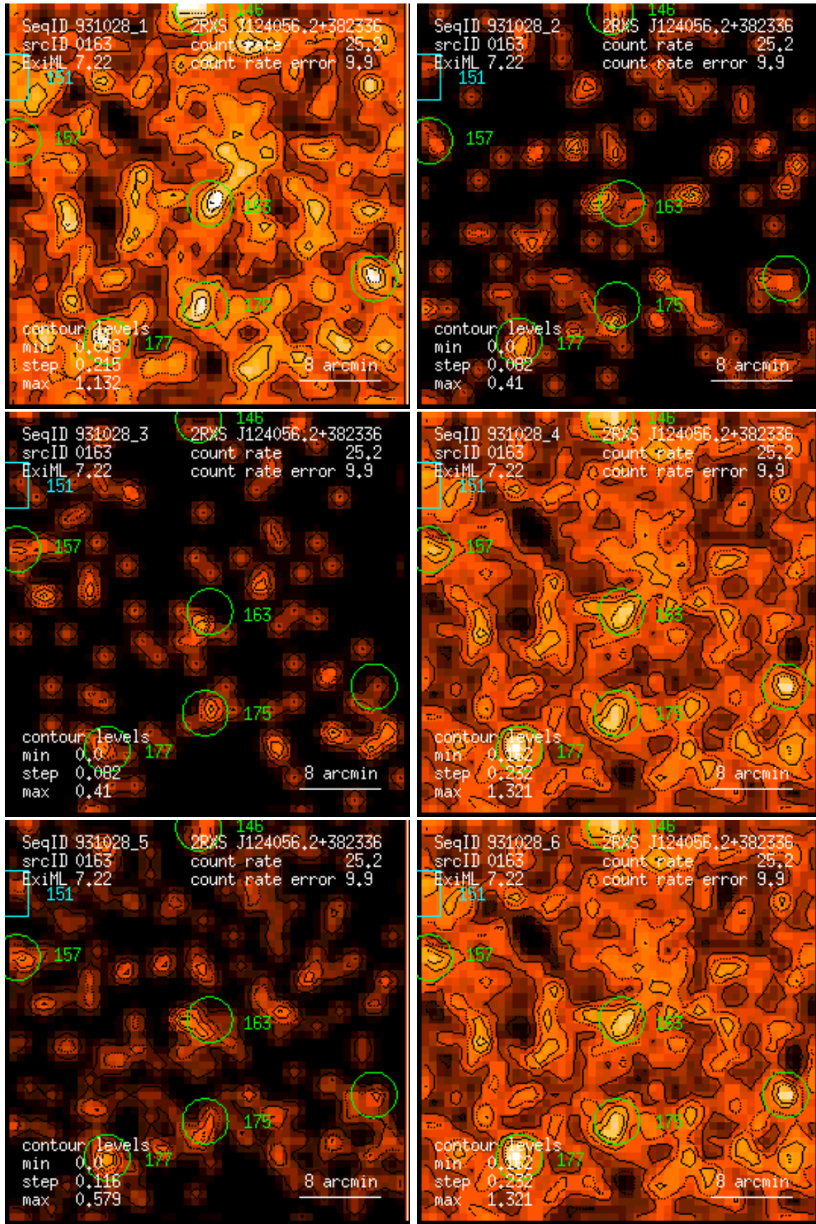
Figure 163: RASS 931028: detection 0163: band rate images, Gaussian filter: (1) PSPC channels 11 – 41, (2) 52 – 90, (3) 91 – 201, (4) 11 – 235, (5) 52 – 201, (6) 11 – 201. Broad band rates in counts/ks. Band rate contour levels in counts/ks/arcmin 2 .
