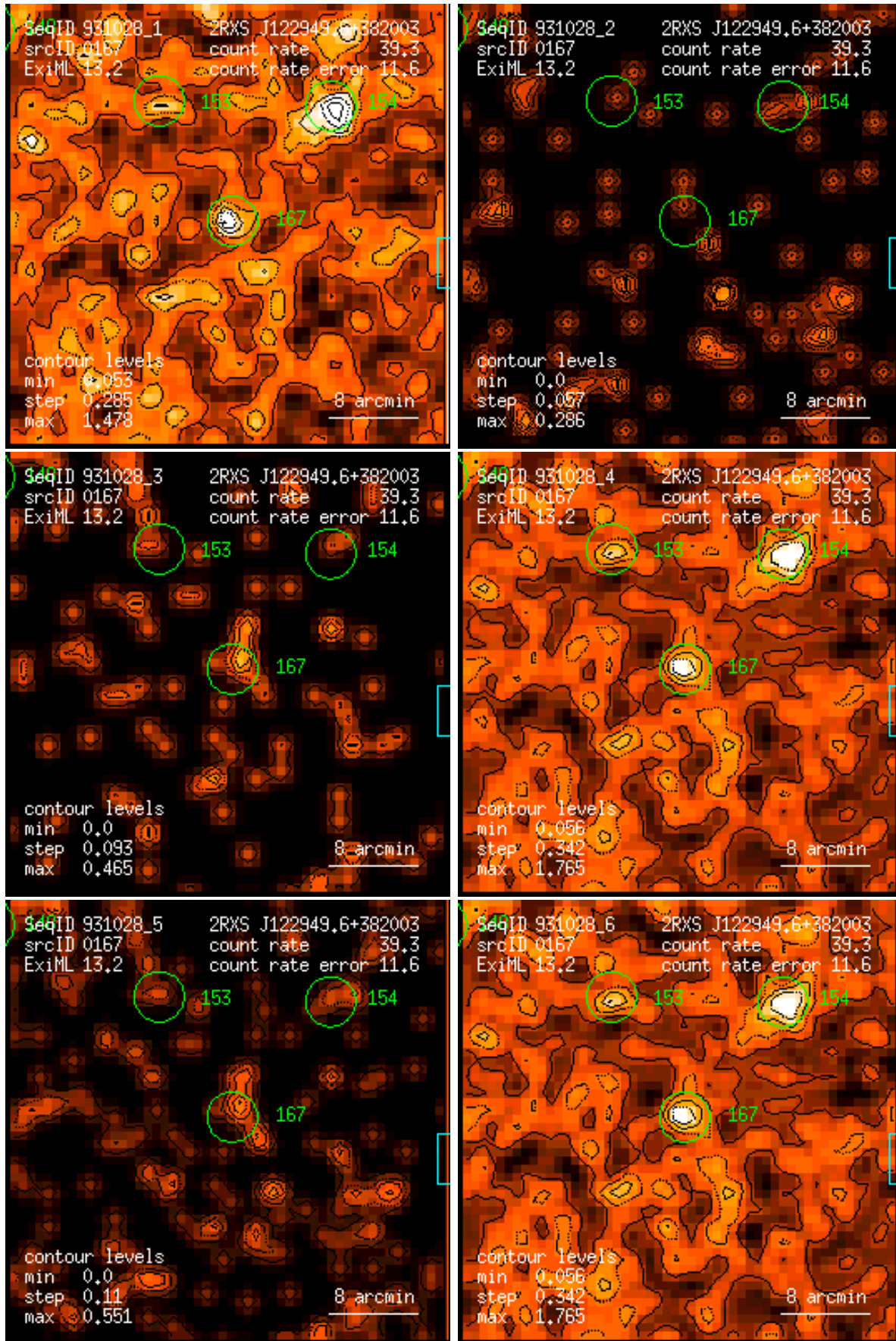
Figure 167: RASS 931028: detection 0167: band rate images, Gaussian filter: (1) PSPC channels 11 – 41, (2) 52 – 90, (3) 91 – 201, (4) 11 – 235, (5) 52 – 201, (6) 11 – 201. Broad band rates in counts/ks. Band rate contour levels in counts/ks/arcmin 2 .
