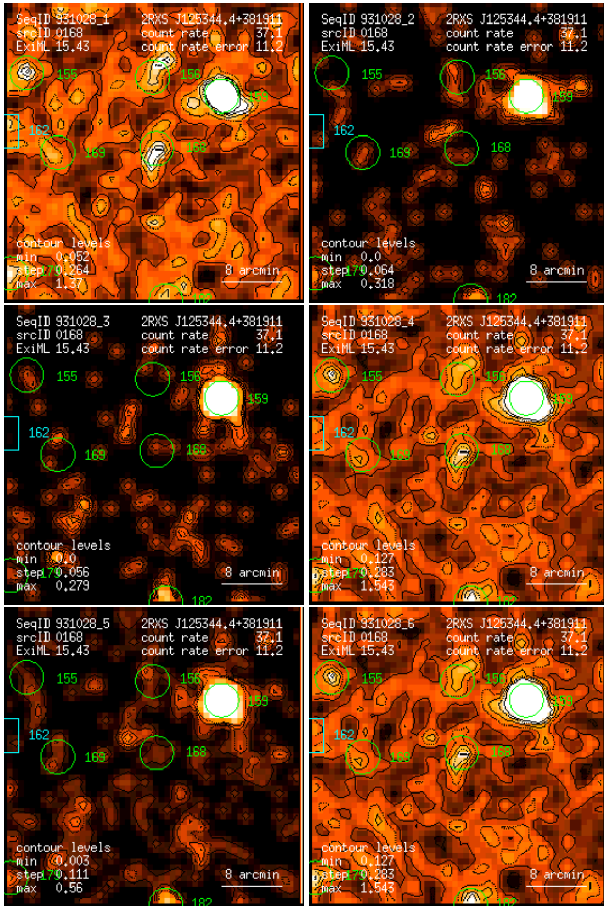
Figure 168: RASS 931028: detection 0168: band rate images, Gaussian filter: (1) PSPC channels 11 – 41, (2) 52 – 90, (3) 91 – 201, (4) 11 – 235, (5) 52 – 201, (6) 11 – 201. Broad band rates in counts/ks. Band rate contour levels in counts/ks/arcmin 2 .
