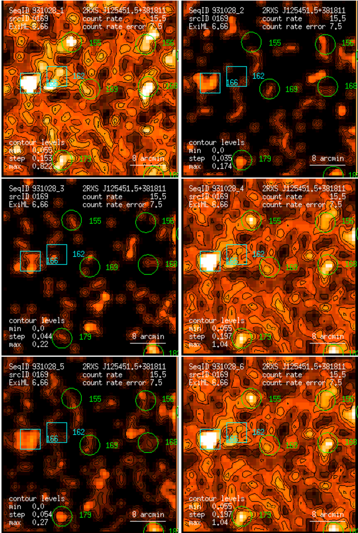
Figure 169: RASS 931028: detection 0169: band rate images, Gaussian filter: (1) PSPC channels 11 – 41, (2) 52 – 90, (3) 91 – 201, (4) 11 – 235, (5) 52 – 201, (6) 11 – 201. Broad band rates in counts/ks. Band rate contour levels in counts/ks/arcmin 2 .
