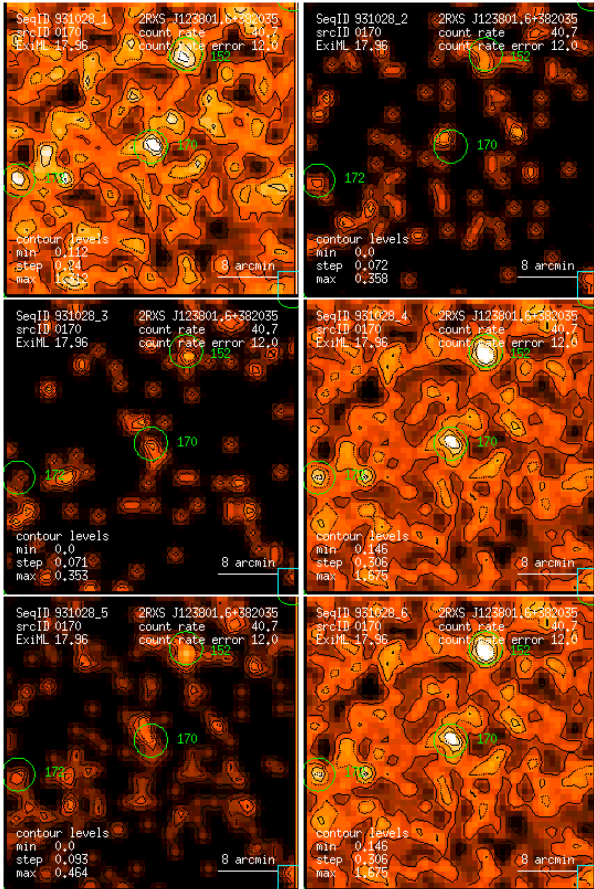
Figure 170: RASS 931028: detection 0170: band rate images, Gaussian filter: (1) PSPC channels 11 – 41, (2) 52 – 90, (3) 91 – 201, (4) 11 – 235, (5) 52 – 201, (6) 11 – 201. Broad band rates in counts/ks. Band rate contour levels in counts/ks/arcmin 2 .
