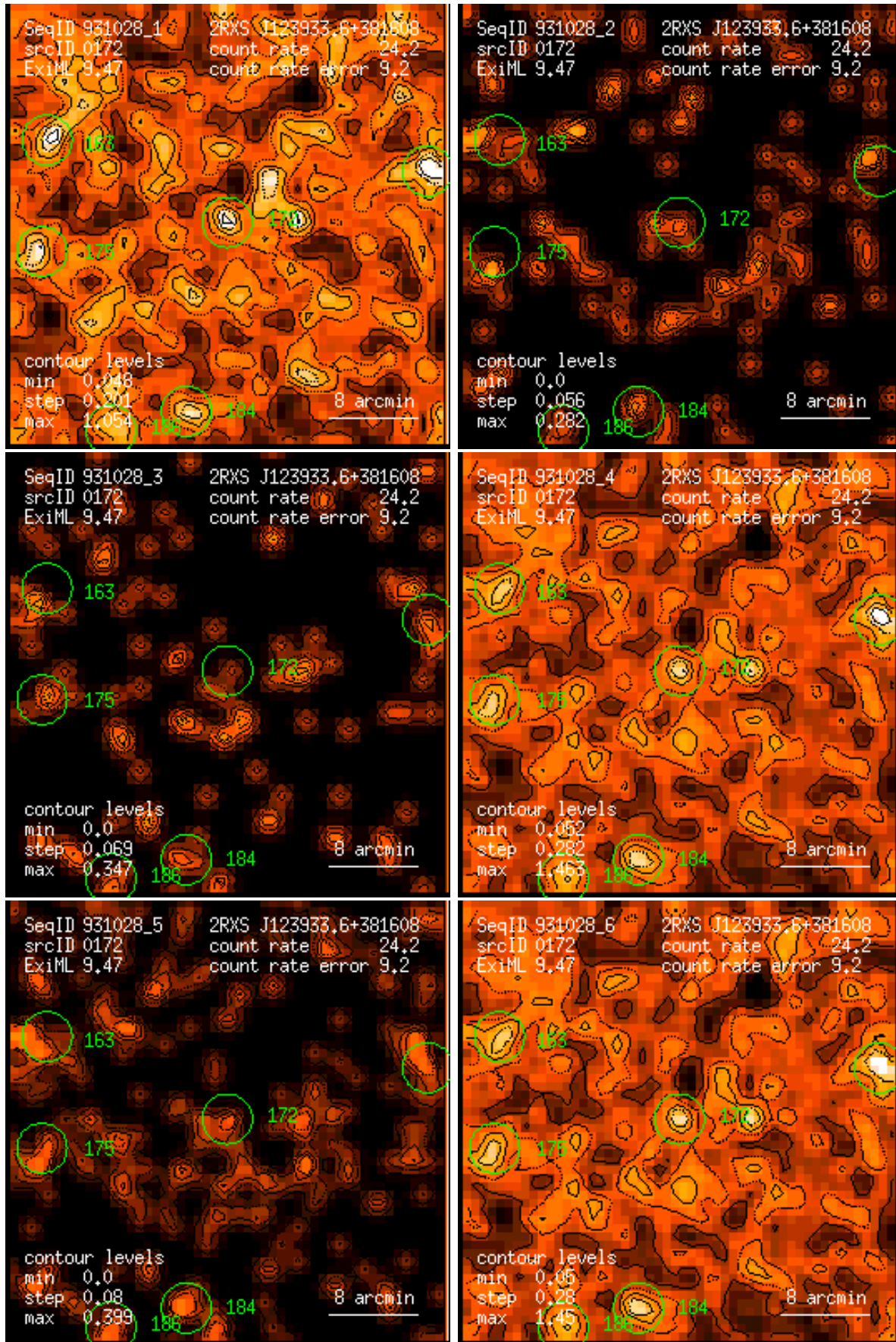
Figure 172: RASS 931028: detection 0172: band rate images, Gaussian filter: (1) PSPC channels 11 – 41, (2) 52 – 90, (3) 91 – 201, (4) 11 – 235, (5) 52 – 201, (6) 11 – 201. Broad band rates in counts/ks. Band rate contour levels in counts/ks/arcmin 2 .
