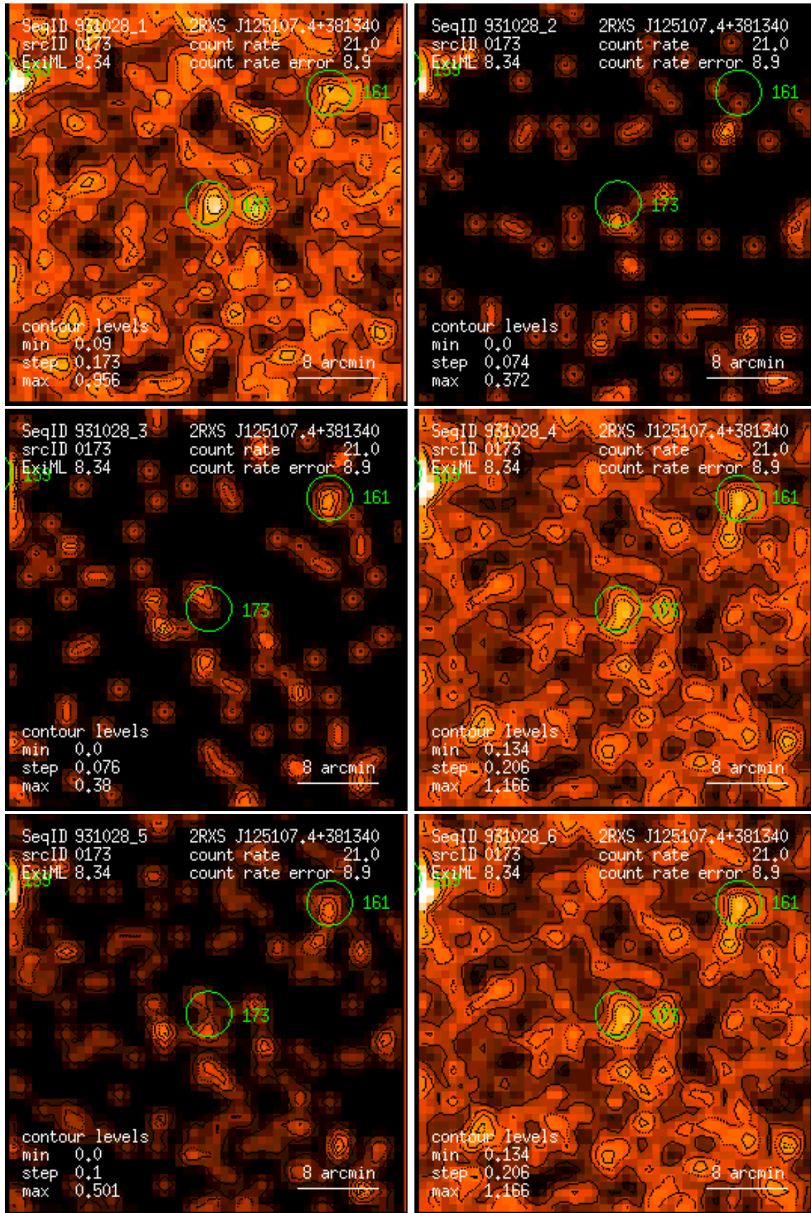
Figure 173: RASS 931028: detection 0173: band rate images, Gaussian filter: (1) PSPC channels 11 – 41, (2) 52 – 90, (3) 91 – 201, (4) 11 – 235, (5) 52 – 201, (6) 11 – 201. Broad band rates in counts/ks. Band rate contour levels in counts/ks/arcmin 2 .
