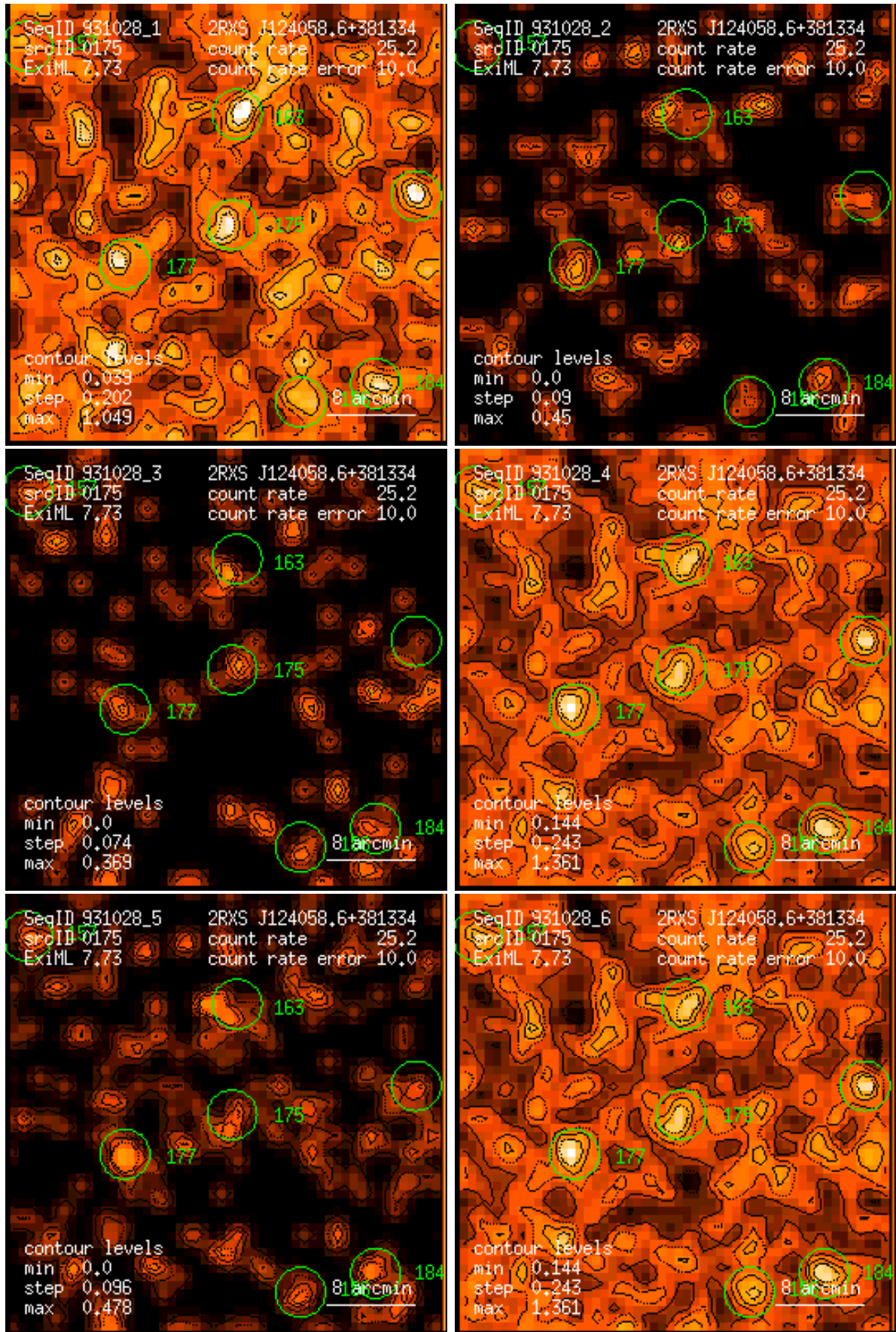
Figure 175: RASS 931028: detection 0175: band rate images, Gaussian filter: (1) PSPC channels 11 – 41, (2) 52 – 90, (3) 91 – 201, (4) 11 – 235, (5) 52 – 201, (6) 11 – 201. Broad band rates in counts/ks. Band rate contour levels in counts/ks/arcmin 2 .
