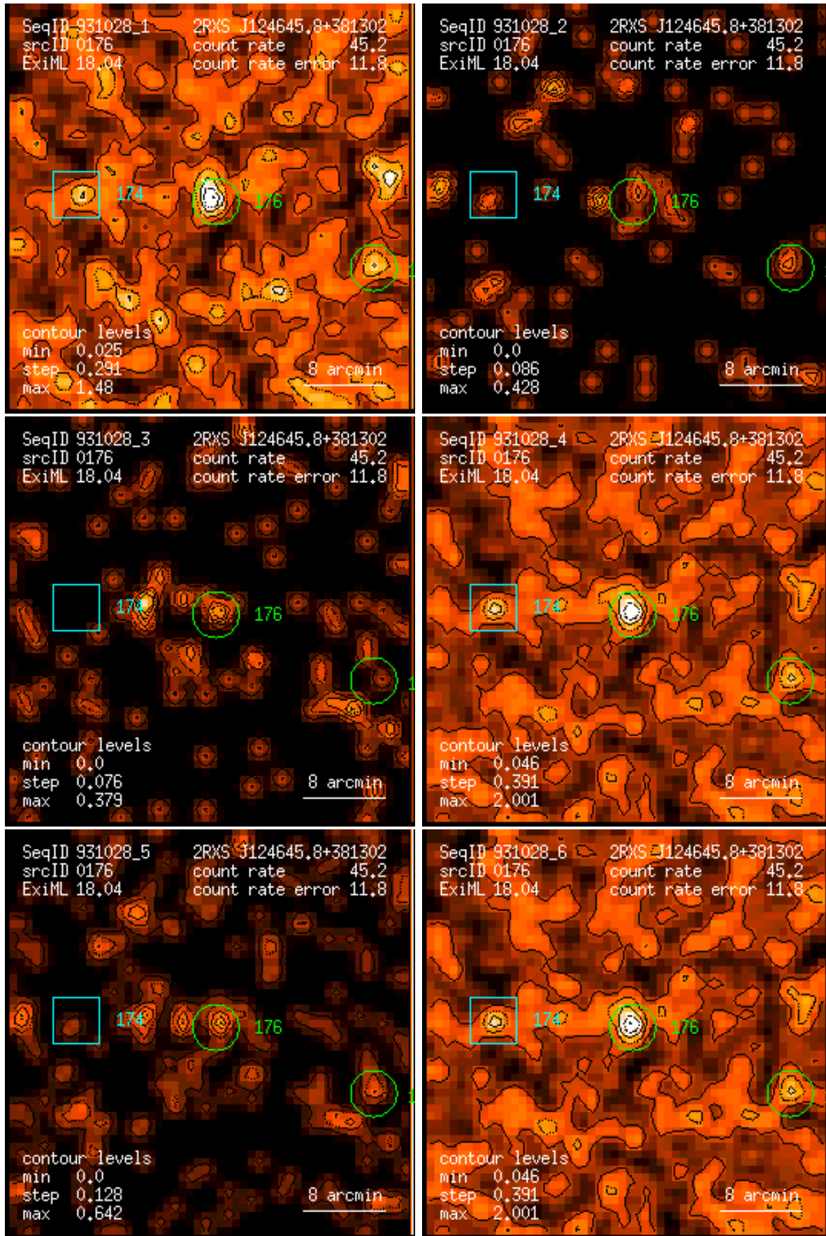
Figure 176: RASS 931028: detection 0176: band rate images, Gaussian filter: (1) PSPC channels 11 – 41, (2) 52 – 90, (3) 91 – 201, (4) 11 – 235, (5) 52 – 201, (6) 11 – 201. Broad band rates in counts/ks. Band rate contour levels in counts/ks/arcmin 2 .
