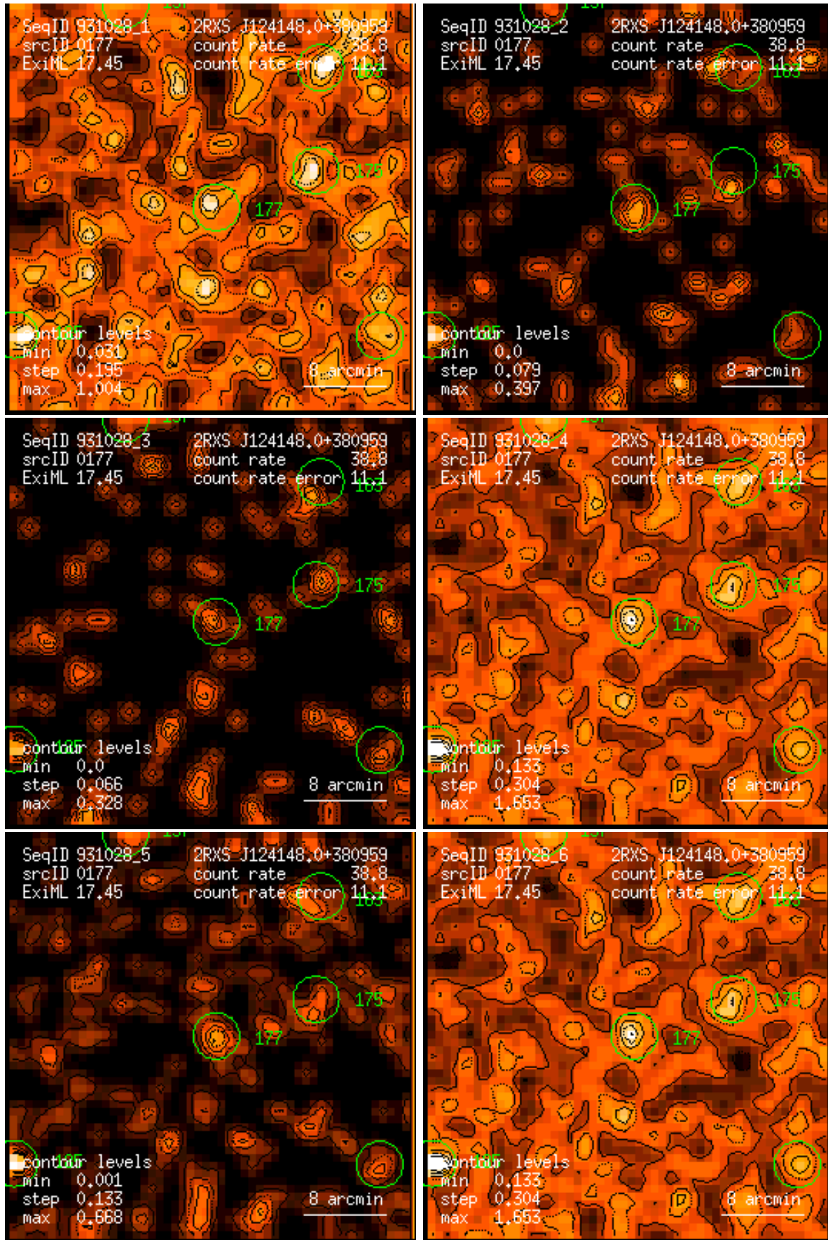
Figure 177: RASS 931028: detection 0177: band rate images, Gaussian filter: (1) PSPC channels 11 – 41, (2) 52 – 90, (3) 91 – 201, (4) 11 – 235, (5) 52 – 201, (6) 11 – 201. Broad band rates in counts/ks. Band rate contour levels in counts/ks/arcmin 2 .
