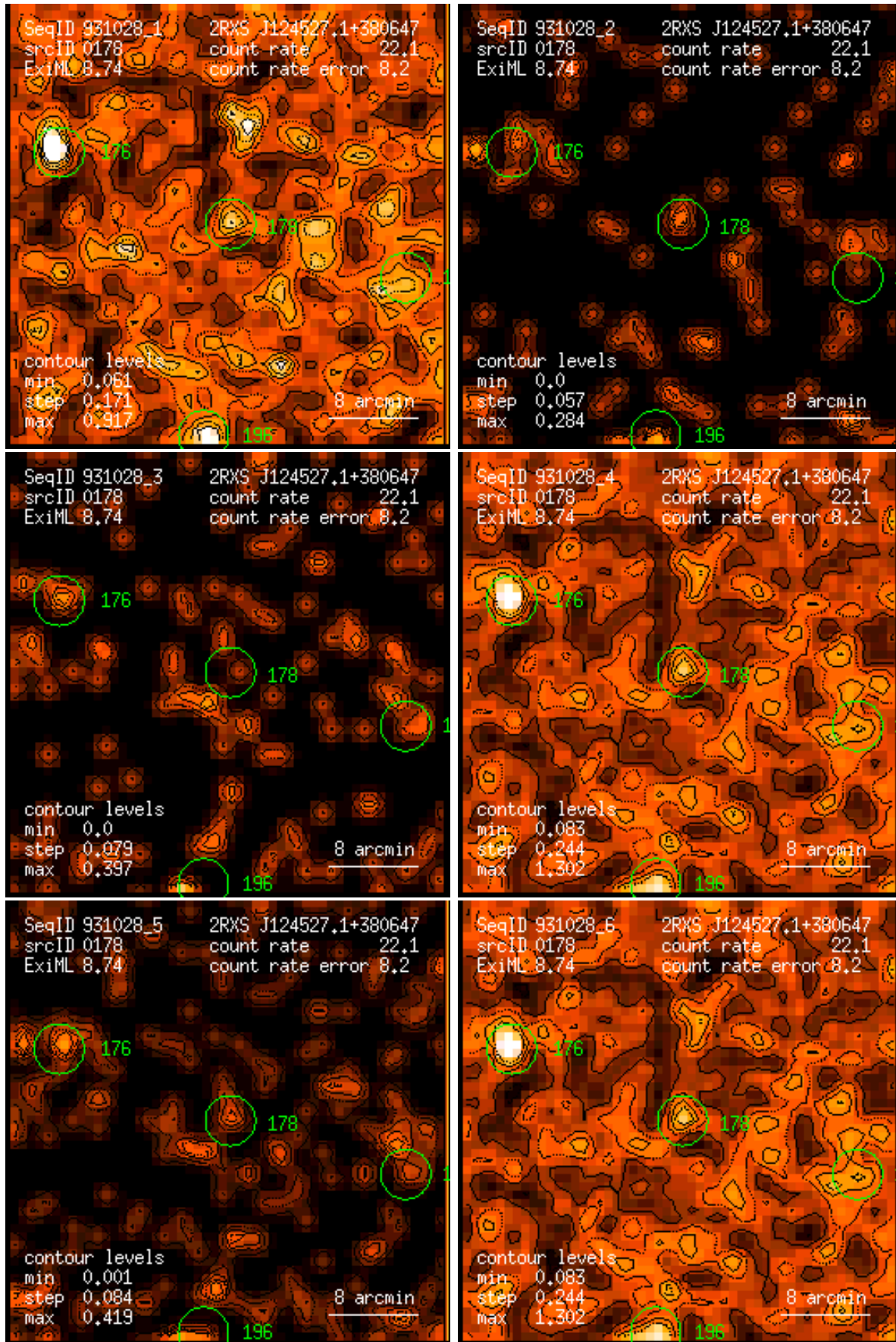
Figure 178: RASS 931028: detection 0178: band rate images, Gaussian filter: (1) PSPC channels 11 – 41, (2) 52 – 90, (3) 91 – 201, (4) 11 – 235, (5) 52 – 201, (6) 11 – 201. Broad band rates in counts/ks. Band rate contour levels in counts/ks/arcmin 2 .
