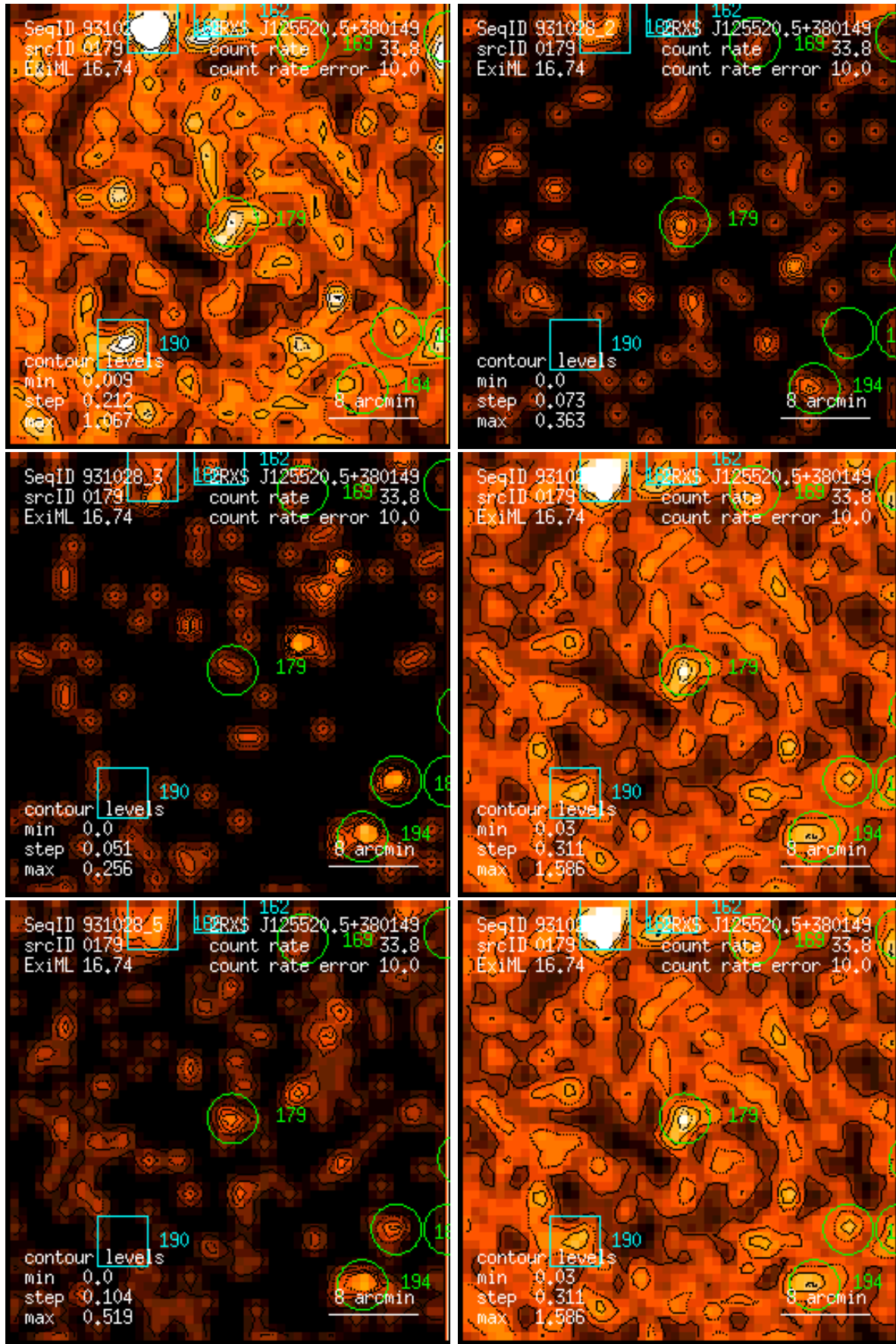
Figure 179: RASS 931028: detection 0179: band rate images, Gaussian filter: (1) PSPC channels 11 – 41, (2) 52 – 90, (3) 91 – 201, (4) 11 – 235, (5) 52 – 201, (6) 11 – 201. Broad band rates in counts/ks. Band rate contour levels in counts/ks/arcmin 2 .
