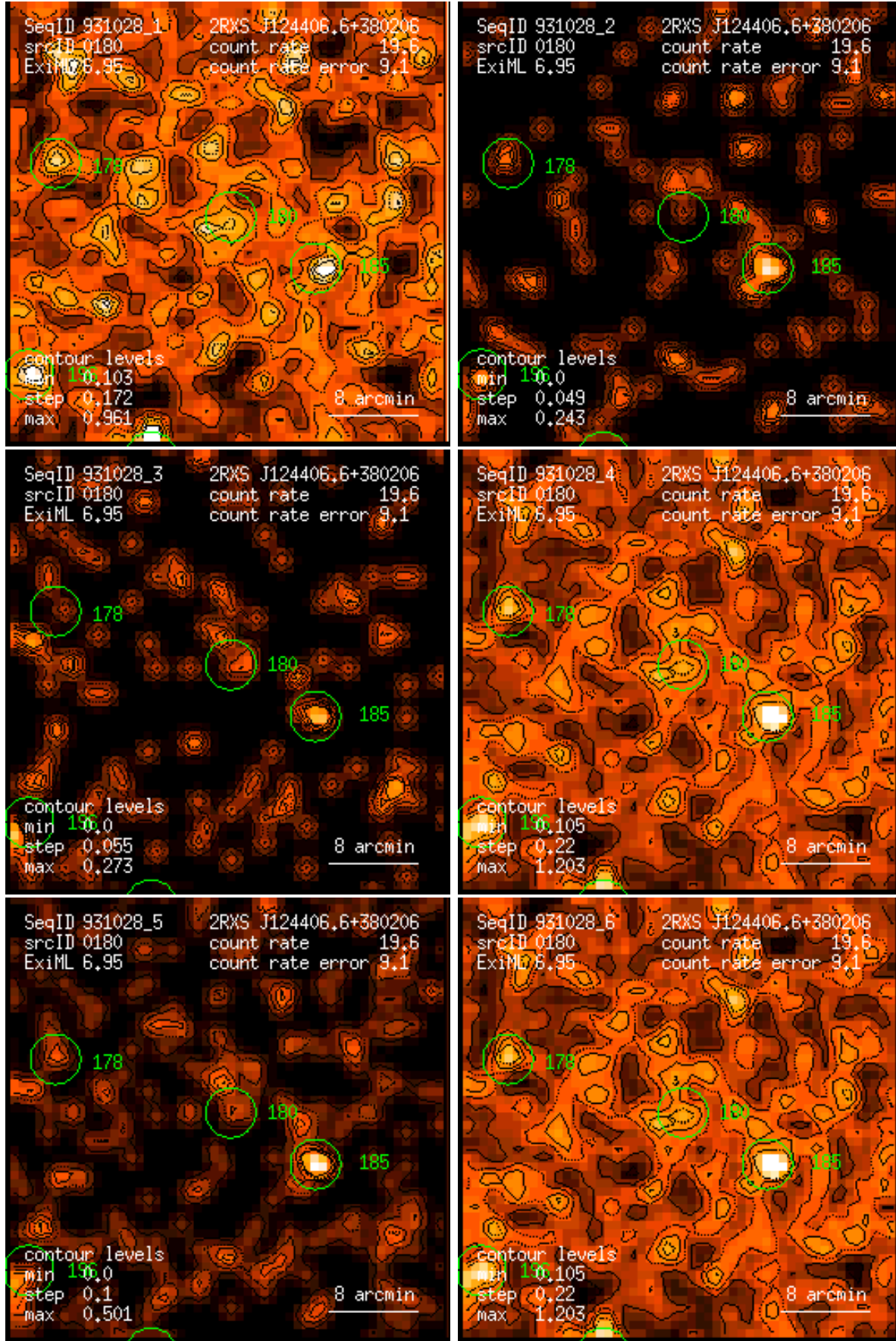
Figure 180: RASS 931028: detection 0180: band rate images, Gaussian filter: (1) PSPC channels 11 – 41, (2) 52 – 90, (3) 91 – 201, (4) 11 – 235, (5) 52 – 201, (6) 11 – 201. Broad band rates in counts/ks. Band rate contour levels in counts/ks/arcmin 2 .
