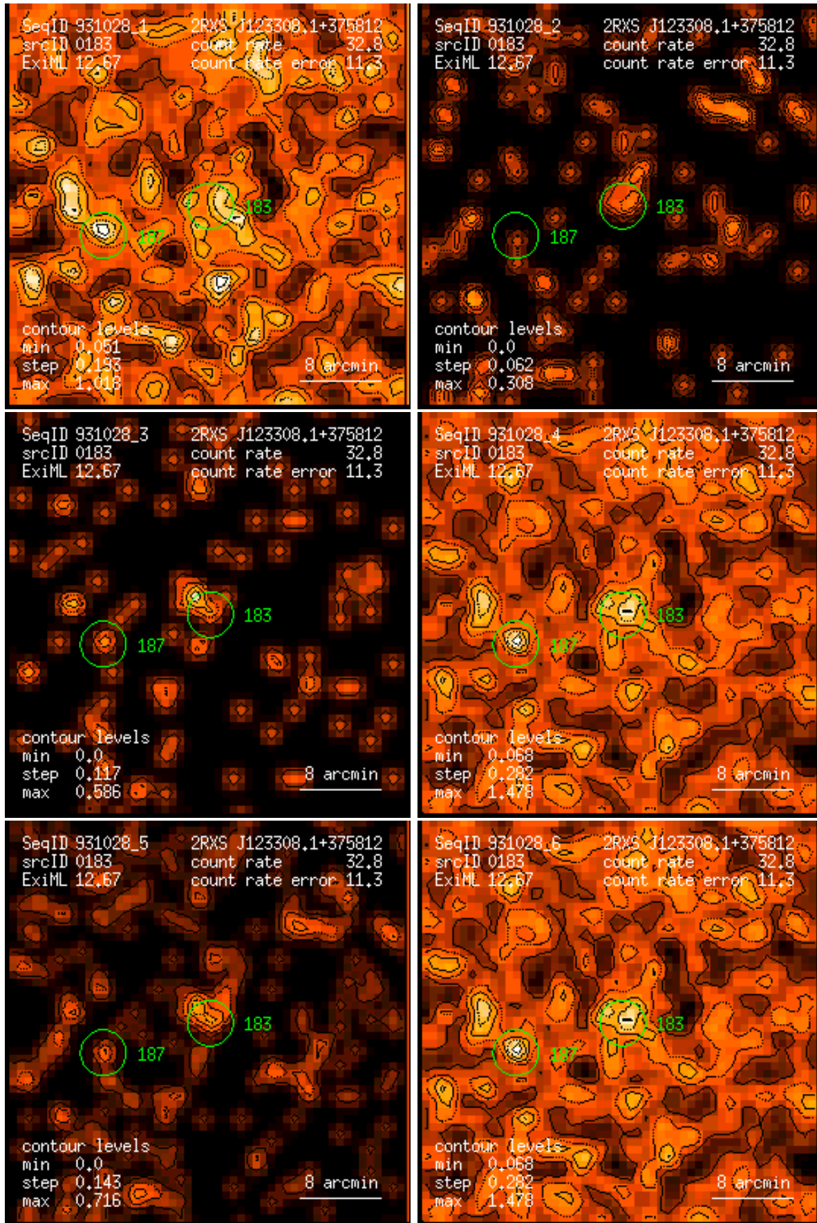
Figure 183: RASS 931028: detection 0183: band rate images, Gaussian filter: (1) PSPC channels 11 – 41, (2) 52 – 90, (3) 91 – 201, (4) 11 – 235, (5) 52 – 201, (6) 11 – 201. Broad band rates in counts/ks. Band rate contour levels in counts/ks/arcmin 2 .
