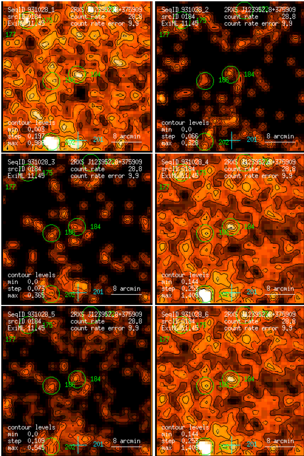
Figure 184: RASS 931028: detection 0184: band rate images, Gaussian filter: (1) PSPC channels 11 – 41, (2) 52 – 90, (3) 91 – 201, (4) 11 – 235, (5) 52 – 201, (6) 11 – 201. Broad band rates in counts/ks. Band rate contour levels in counts/ks/arcmin 2 .
