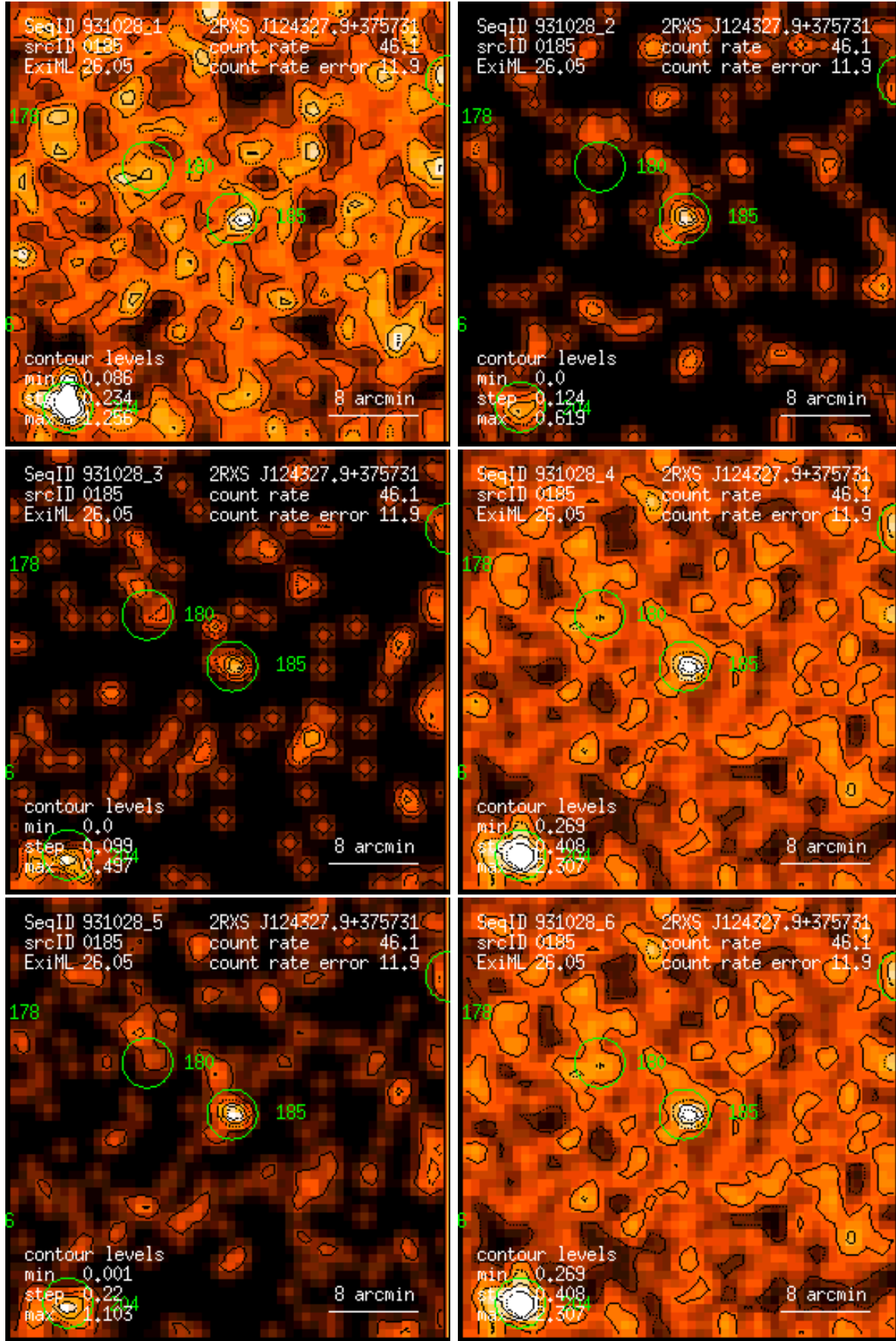
Figure 185: RASS 931028: detection 0185: band rate images, Gaussian filter: (1) PSPC channels 11 – 41, (2) 52 – 90, (3) 91 – 201, (4) 11 – 235, (5) 52 – 201, (6) 11 – 201. Broad band rates in counts/ks. Band rate contour levels in counts/ks/arcmin 2 .
