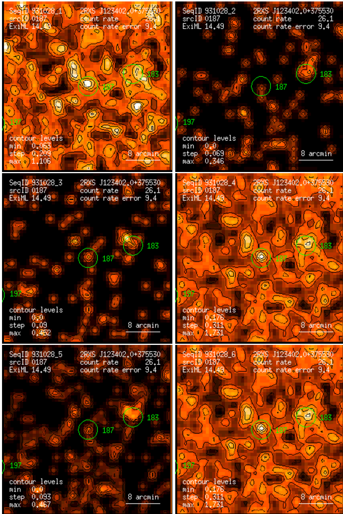
Figure 187: RASS 931028: detection 0187: band rate images, Gaussian filter: (1) PSPC channels 11 – 41, (2) 52 – 90, (3) 91 – 201, (4) 11 – 235, (5) 52 – 201, (6) 11 – 201. Broad band rates in counts/ks. Band rate contour levels in counts/ks/arcmin 2 .
