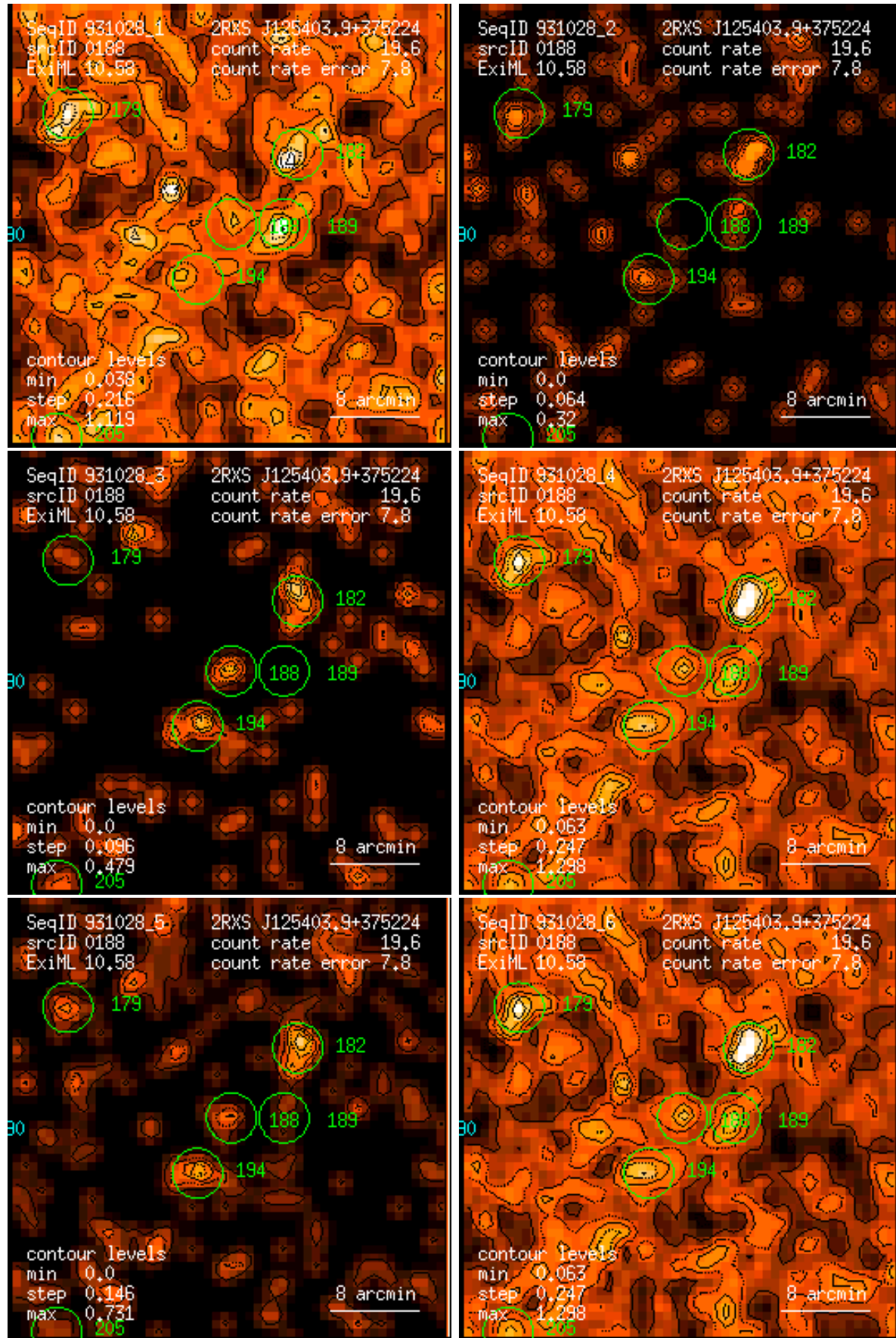
Figure 188: RASS 931028: detection 0188: band rate images, Gaussian filter: (1) PSPC channels 11 – 41, (2) 52 – 90, (3) 91 – 201, (4) 11 – 235, (5) 52 – 201, (6) 11 – 201. Broad band rates in counts/ks. Band rate contour levels in counts/ks/arcmin 2 .
