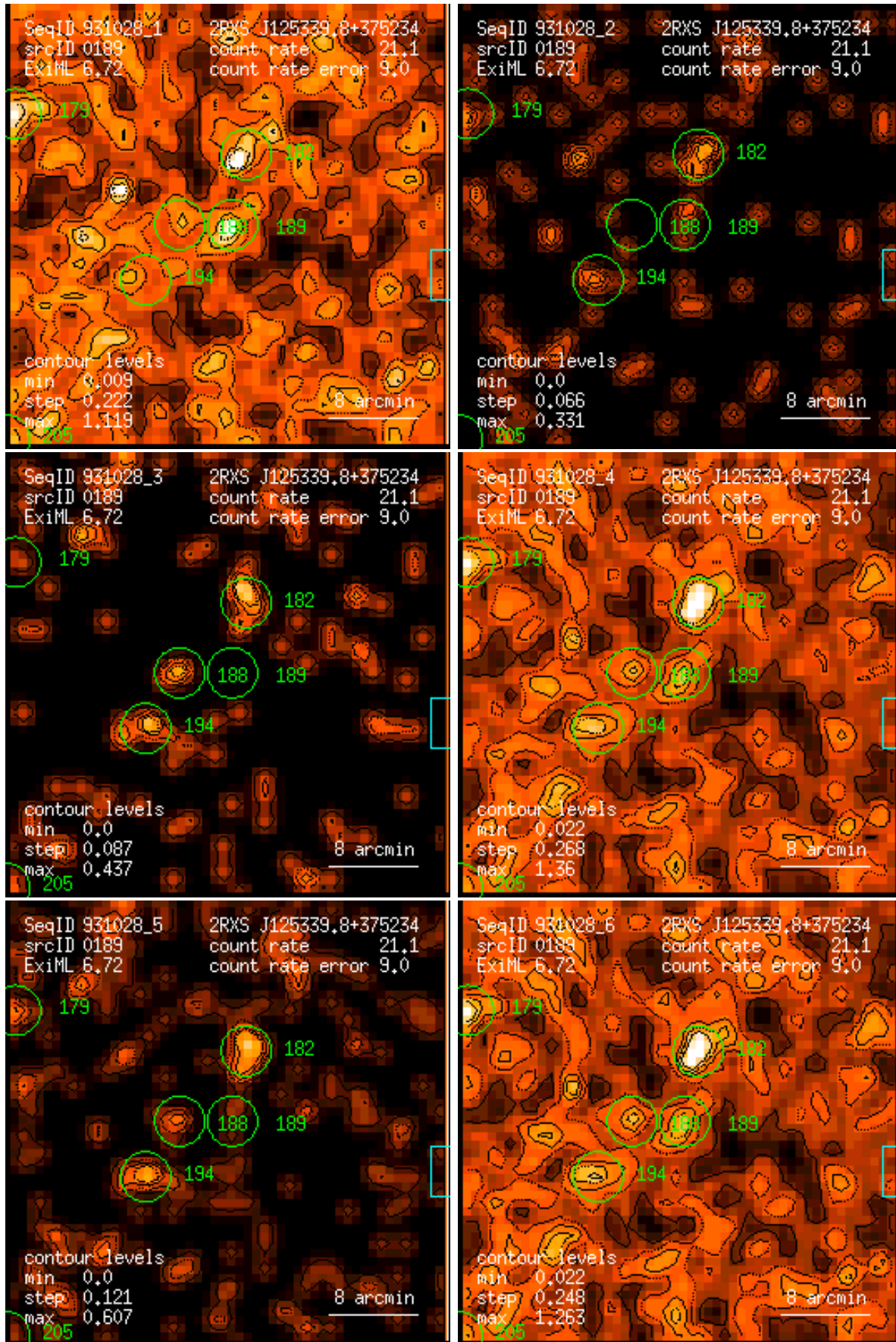
Figure 189: RASS 931028: detection 0189: band rate images, Gaussian filter: (1) PSPC channels 11 – 41, (2) 52 – 90, (3) 91 – 201, (4) 11 – 235, (5) 52 – 201, (6) 11 – 201. Broad band rates in counts/ks. Band rate contour levels in counts/ks/arcmin 2 .
