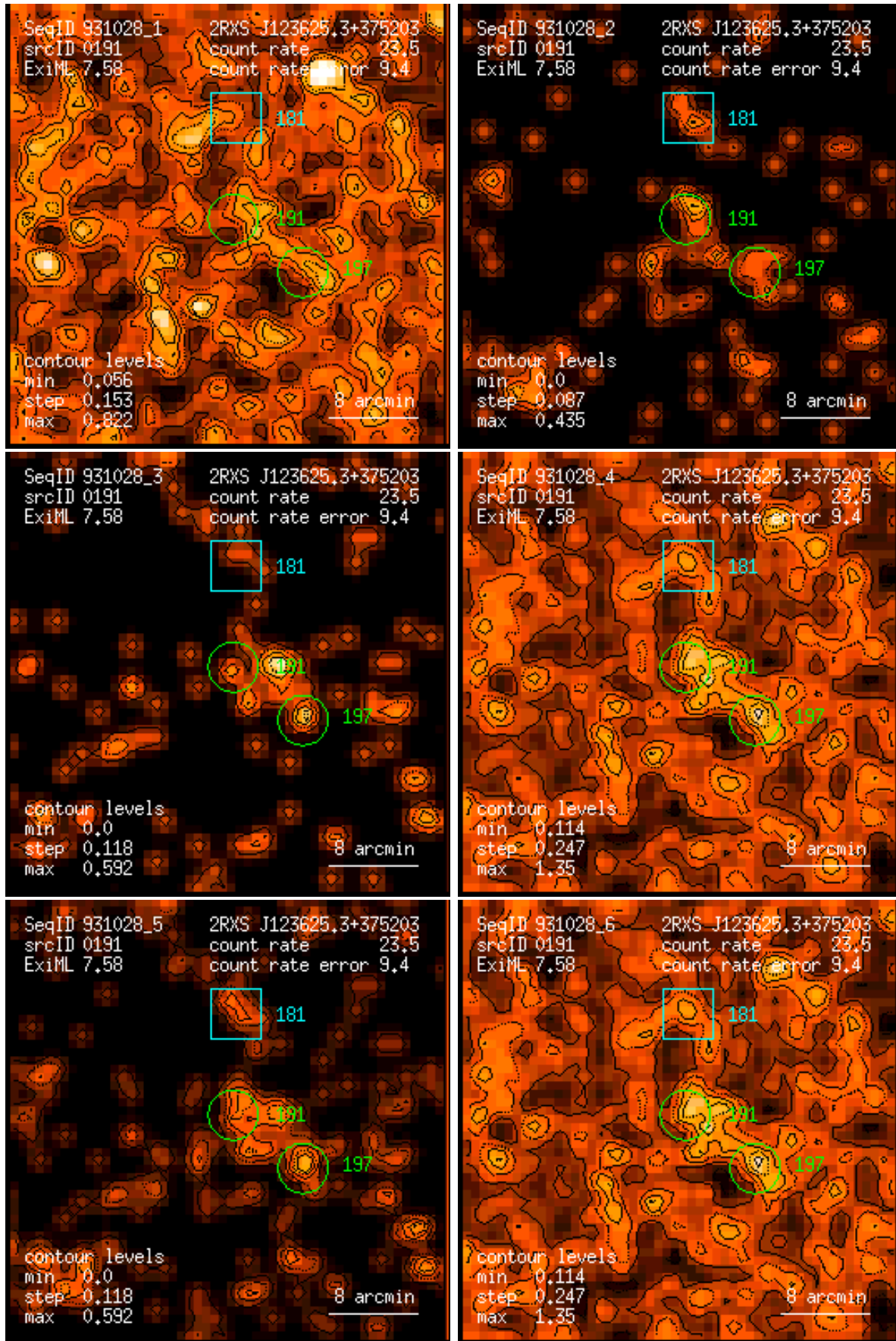
Figure 191: RASS 931028: detection 0191: band rate images, Gaussian filter: (1) PSPC channels 11 – 41, (2) 52 – 90, (3) 91 – 201, (4) 11 – 235, (5) 52 – 201, (6) 11 – 201. Broad band rates in counts/ks. Band rate contour levels in counts/ks/arcmin 2 .
