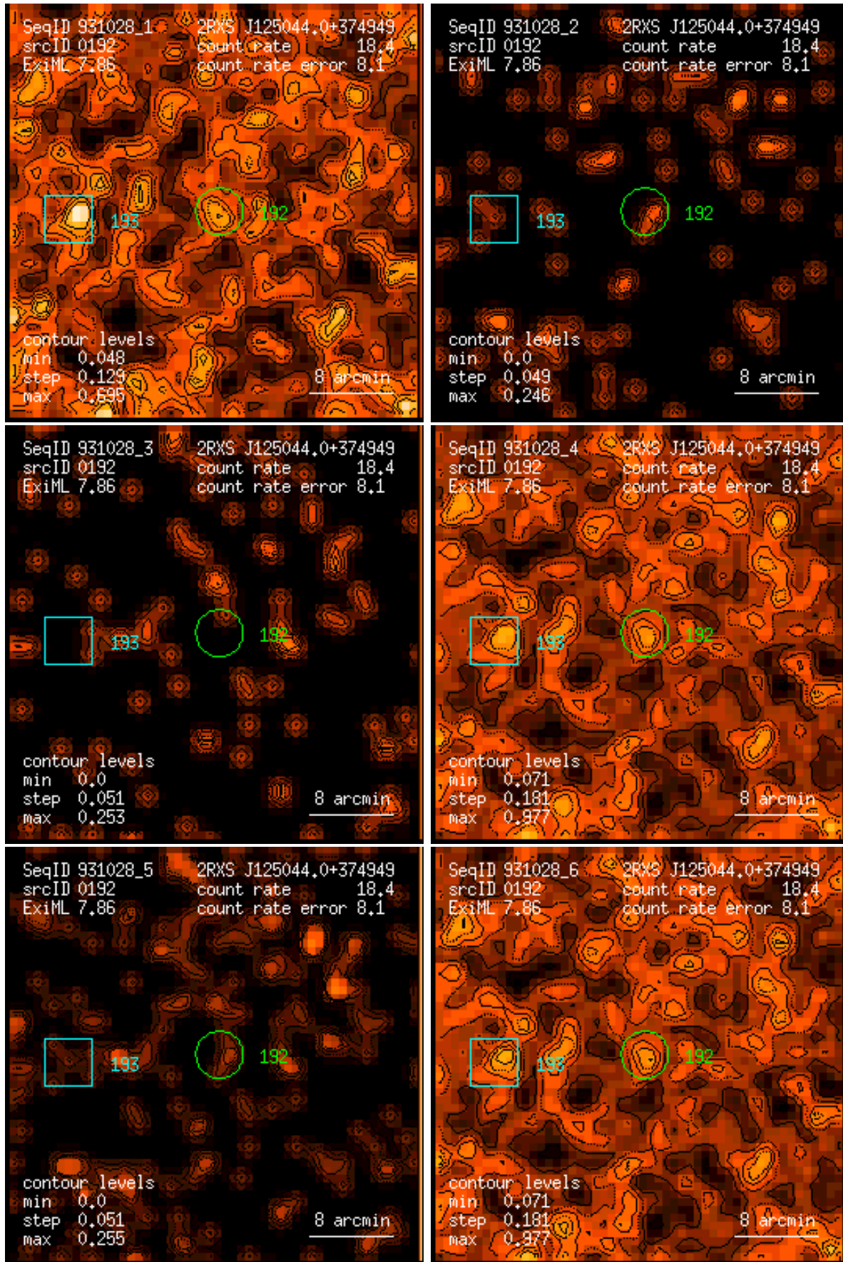
Figure 192: RASS 931028: detection 0192: band rate images, Gaussian filter: (1) PSPC channels 11 – 41, (2) 52 – 90, (3) 91 – 201, (4) 11 – 235, (5) 52 – 201, (6) 11 – 201. Broad band rates in counts/ks. Band rate contour levels in counts/ks/arcmin 2 .
